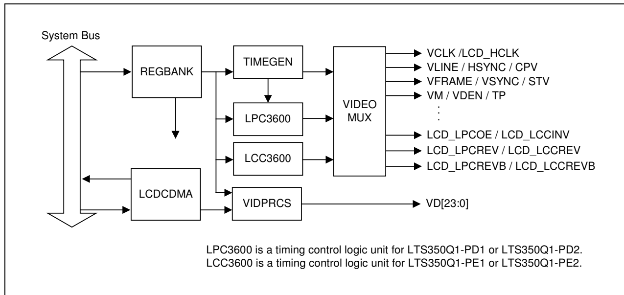
Figure 15-1. LCD Controller Block Diagram
