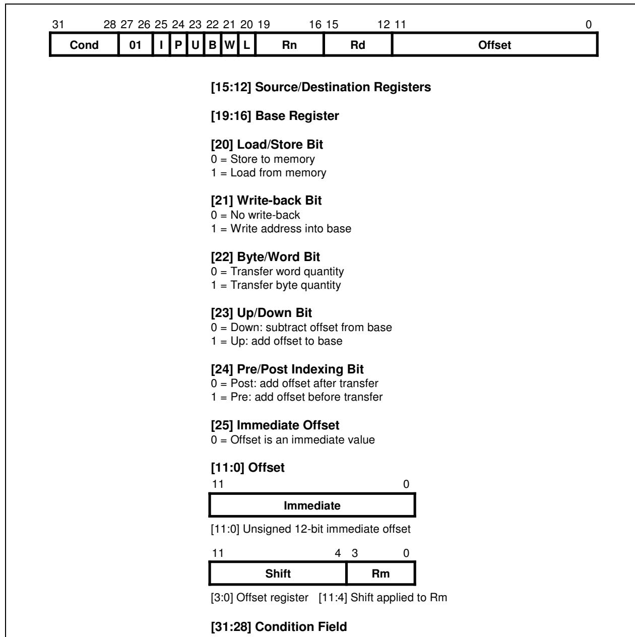
Figure 3-14. Single Data Transfer Instructions
