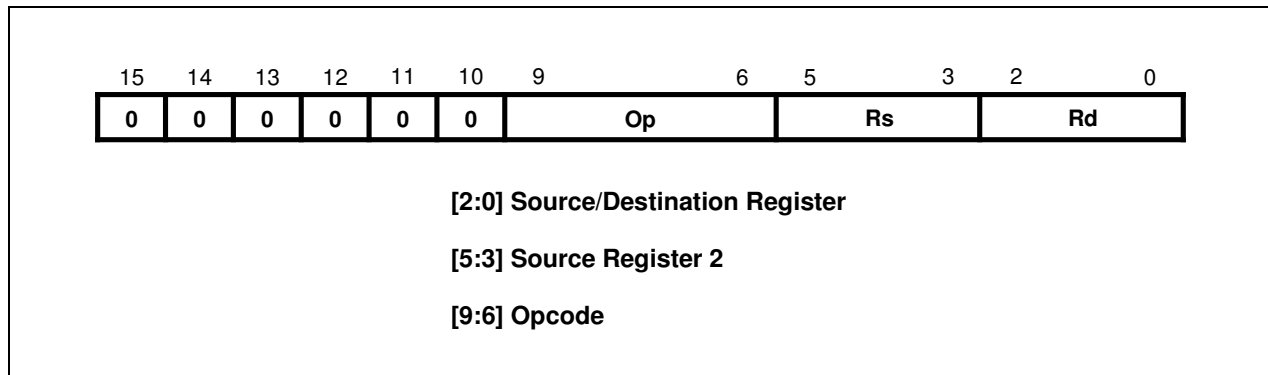
Figure 4-5. Format 4
