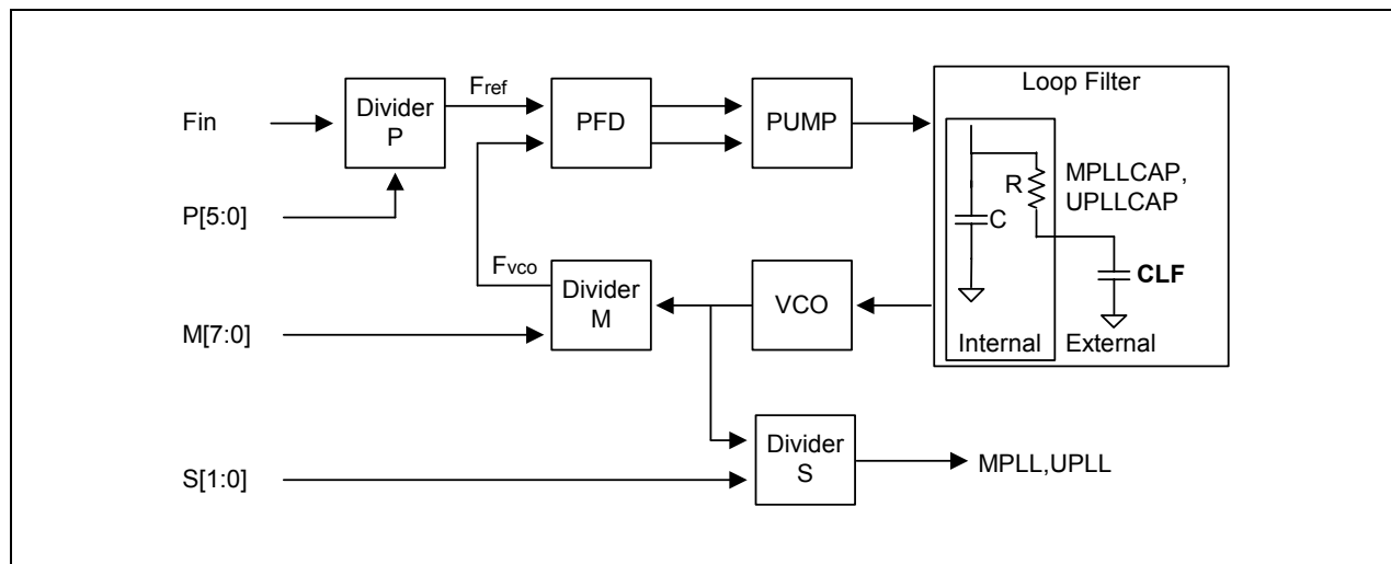
Figure 7-2. PLL (Phase-Locked Loop) Block Diagram
