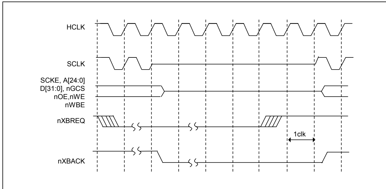
Figure 5-3. S3C2440A nXBREQ/nXBACK Timing Diagram
