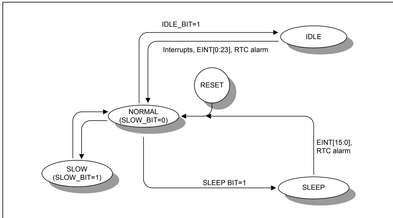
Figure 7-8. Power Management State Diagram
