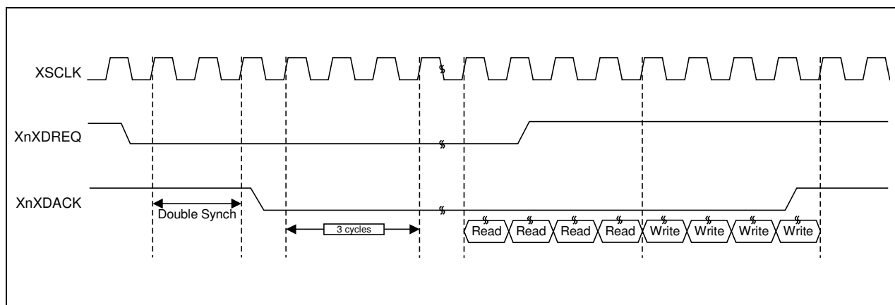
Figure 8-3. Burst 4 Transfer Size
