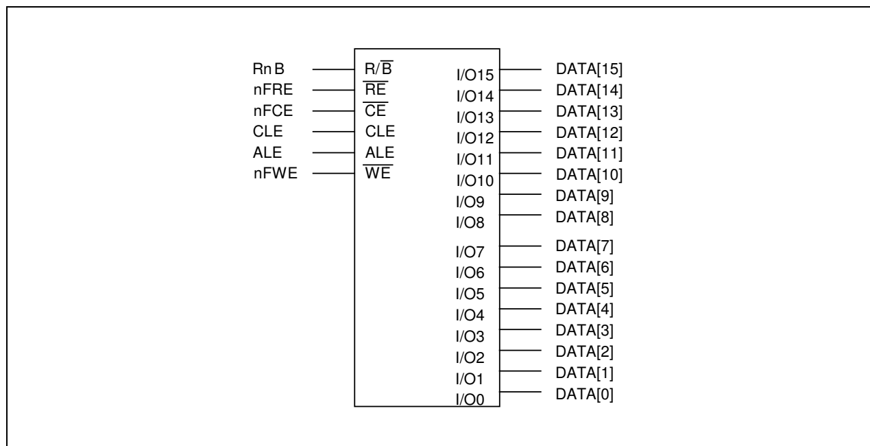
Figure 6-8. A 16-bit NAND Flash Memory Interface
