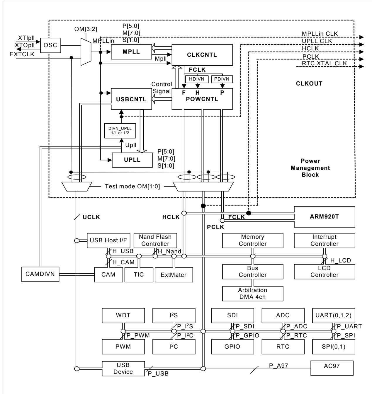
Figure 7-1. Clock Generator Block Diagram
