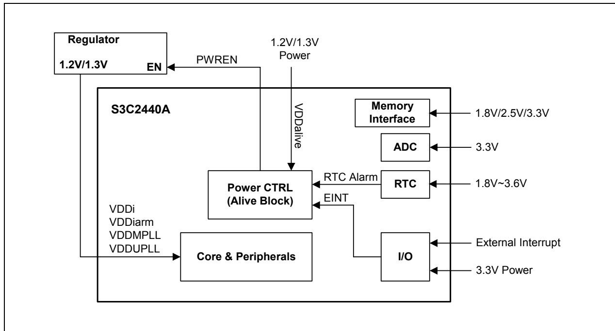
Figure 7-12. SLEEP Mode
