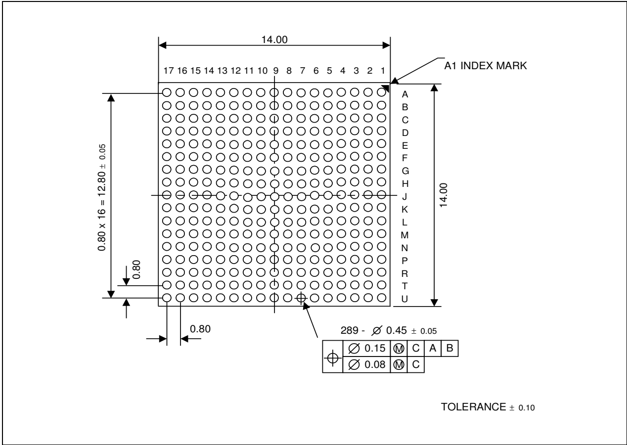
Figure 26-2. 289-FBGA-1414 Package Dimension 2 (Bottom View)
