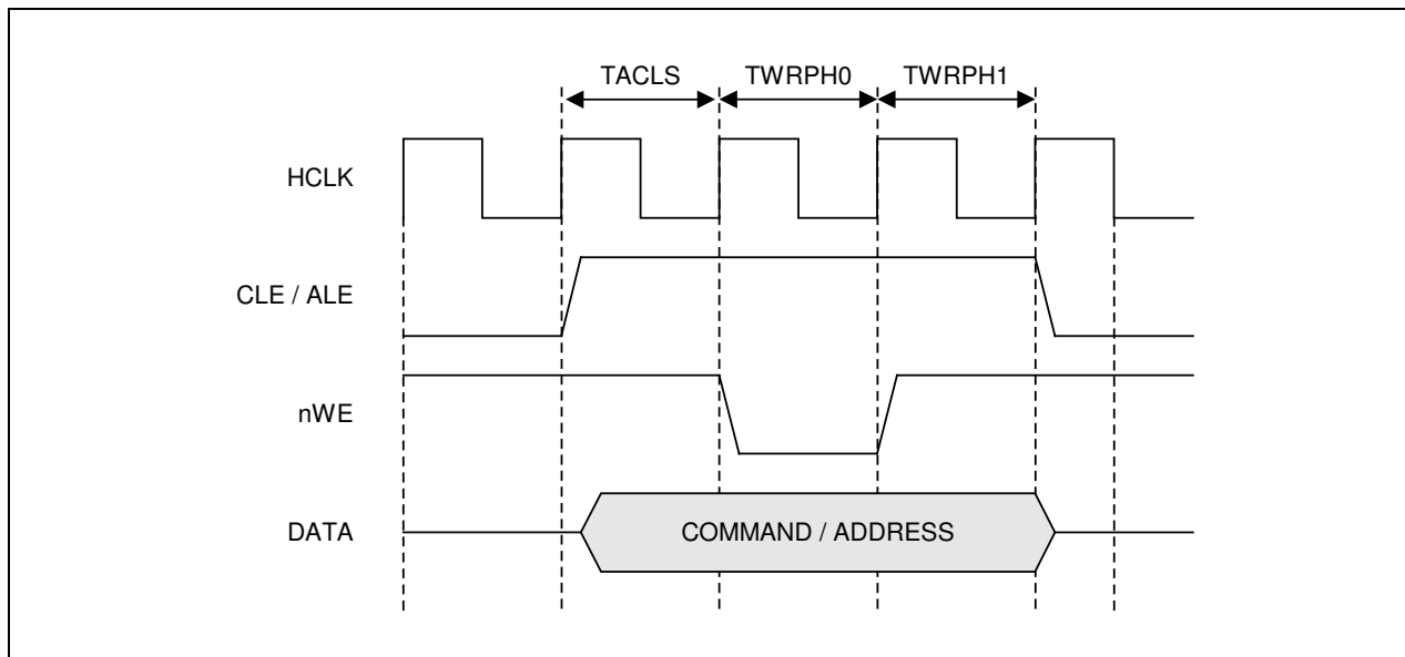
Figure 6-3. CLE &amp; ALE Timing (TACLS=1, TWRPH0=0, TWRPH1=0)
