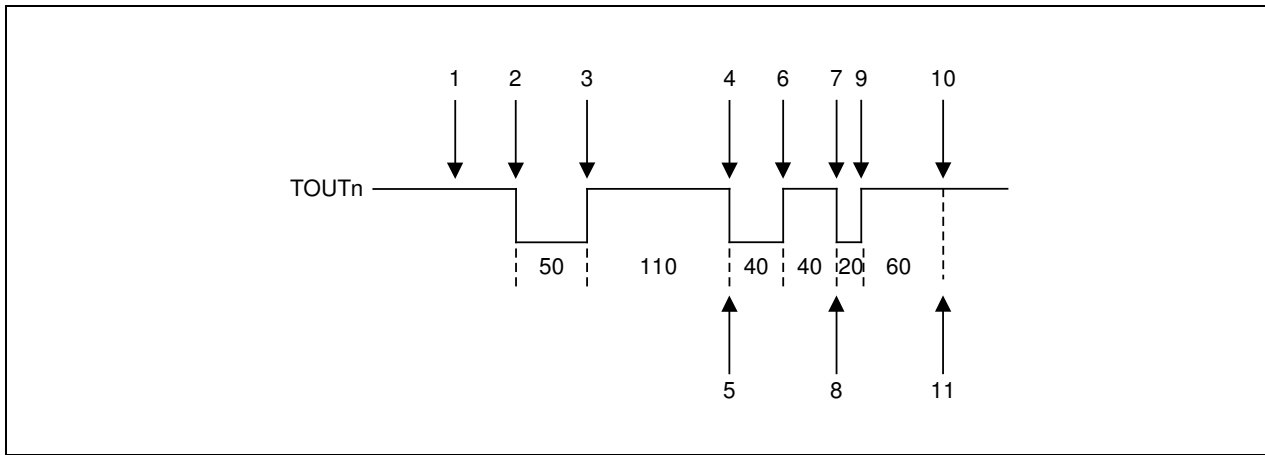
Figure 10-4. Example of a Timer Operation
