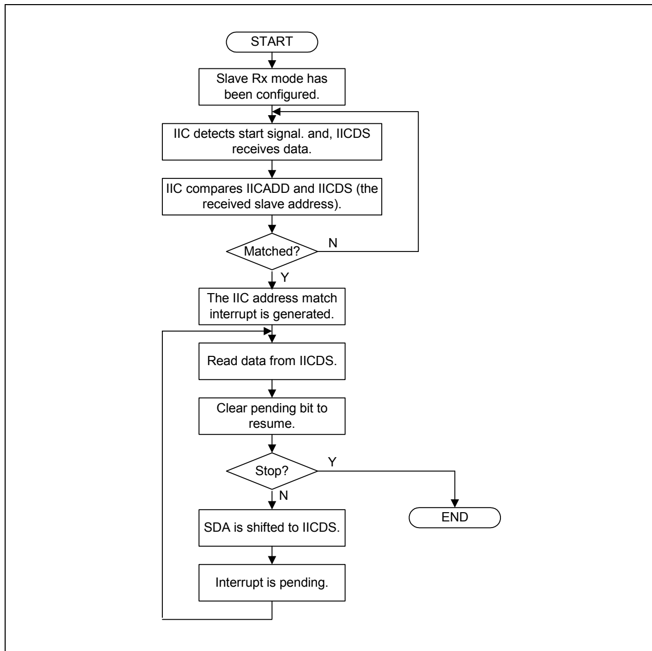
Figure 20-9. Operations for Slave/Receiver Mode
