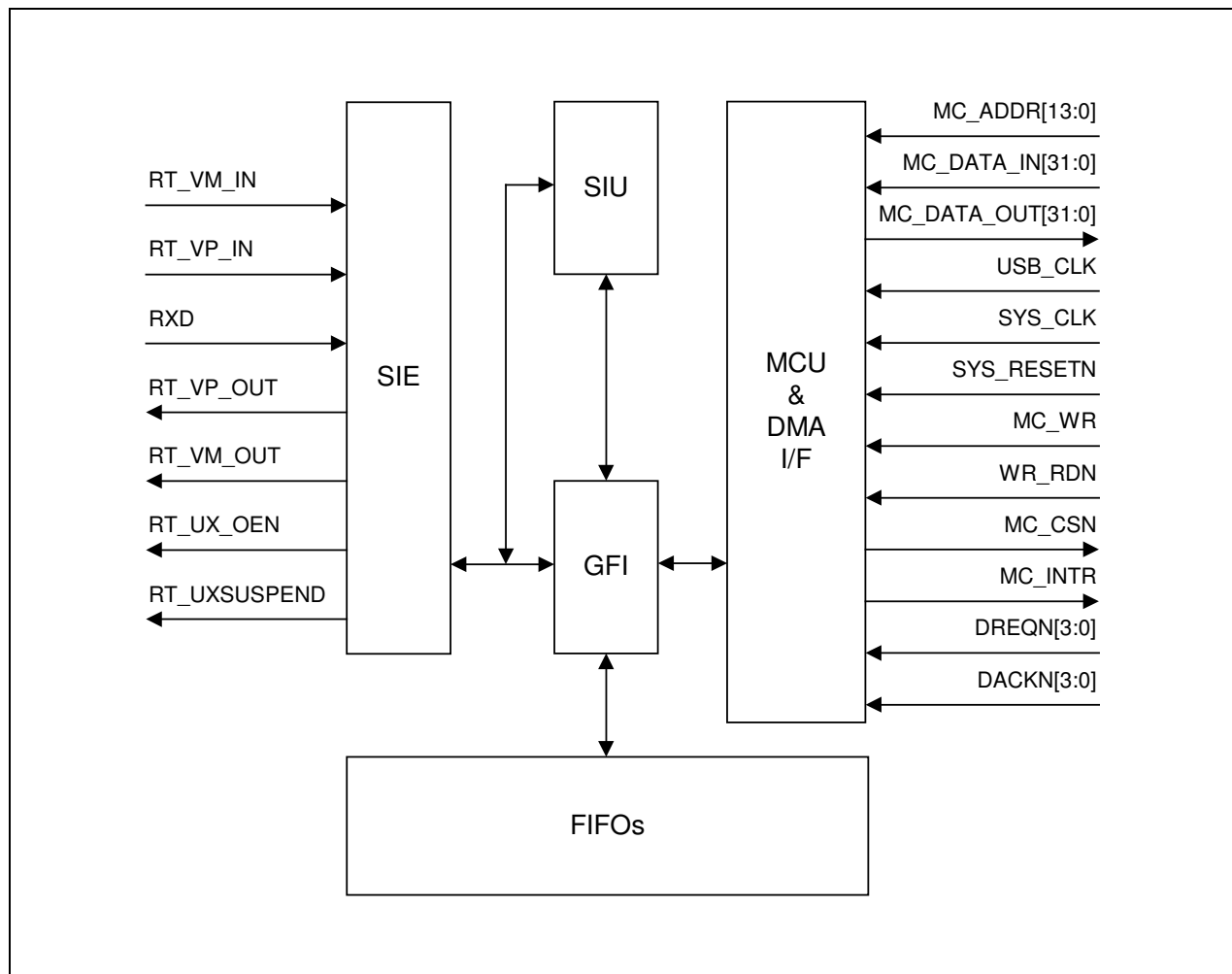
Figure 13-1. USB Device Controller Block Diagram
