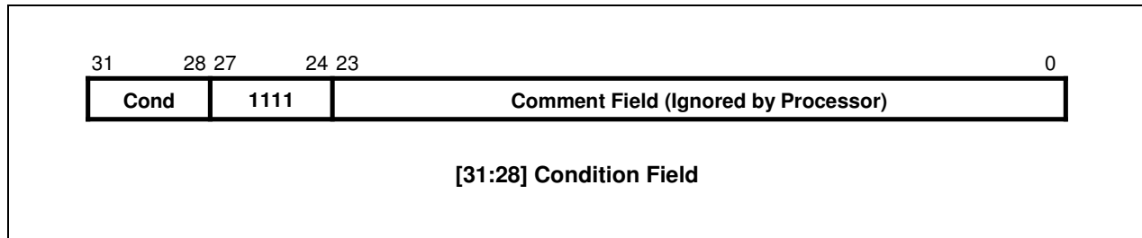
Figure 3-24. Software Interrupt Instruction
