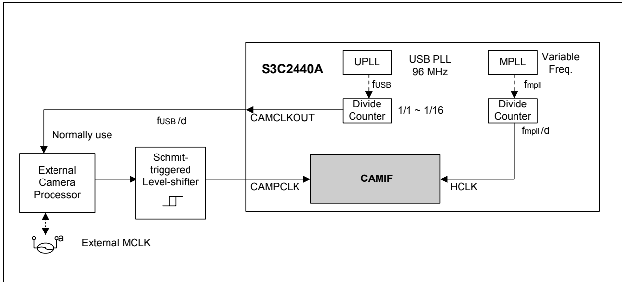
Figure 23-5. CAMIF Clock Generation
