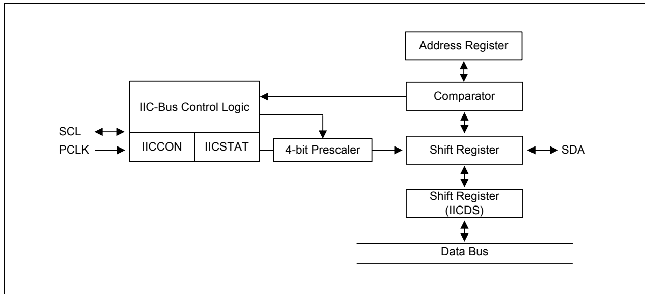
Figure 20-1. IIC-Bus Block Diagram
