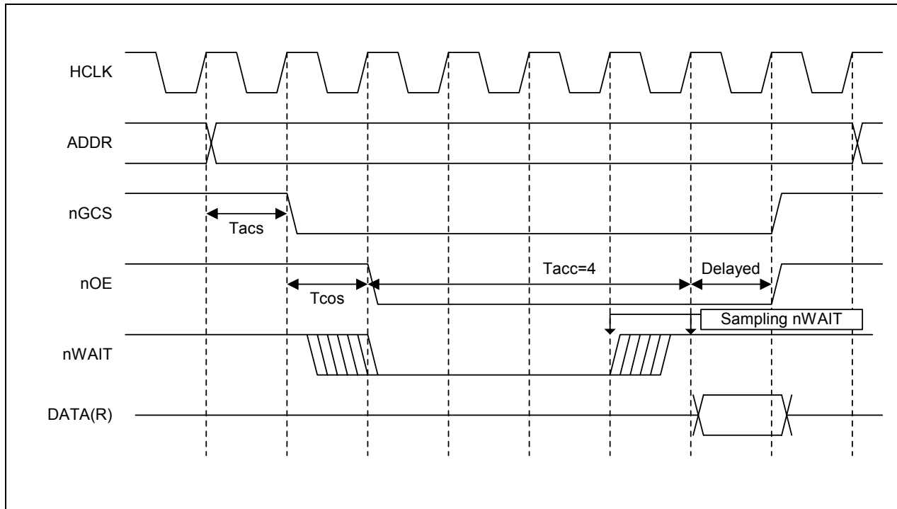
Figure 5-2. S3C2440A External nWAIT Timing Diagram ( T_{acc}=4 )
