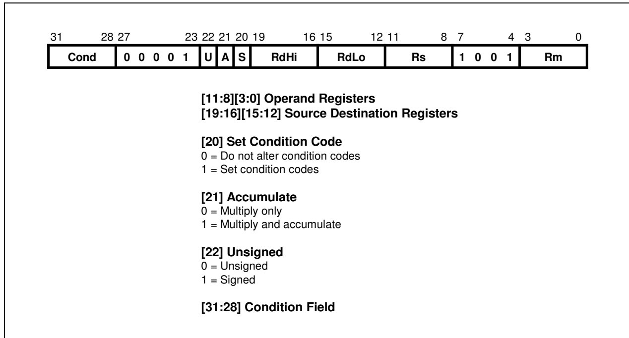
Figure 3-13. Multiply Long Instructions
