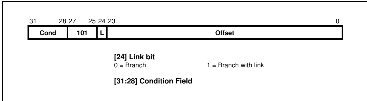
Figure 3-3. Branch Instructions
