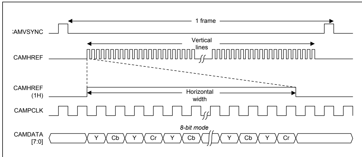
Figure 23-2. ITU-R BT 601 Input Timing Diagram
