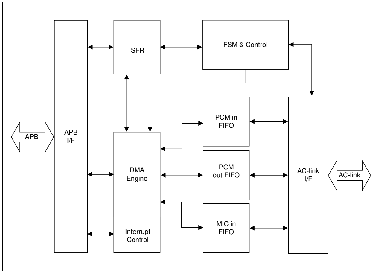
Figure 24-1. AC97 Block Diagram
