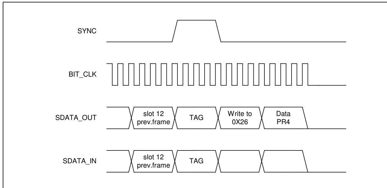
Figure 24-7. AC97 Powerdown Timing Diagram
