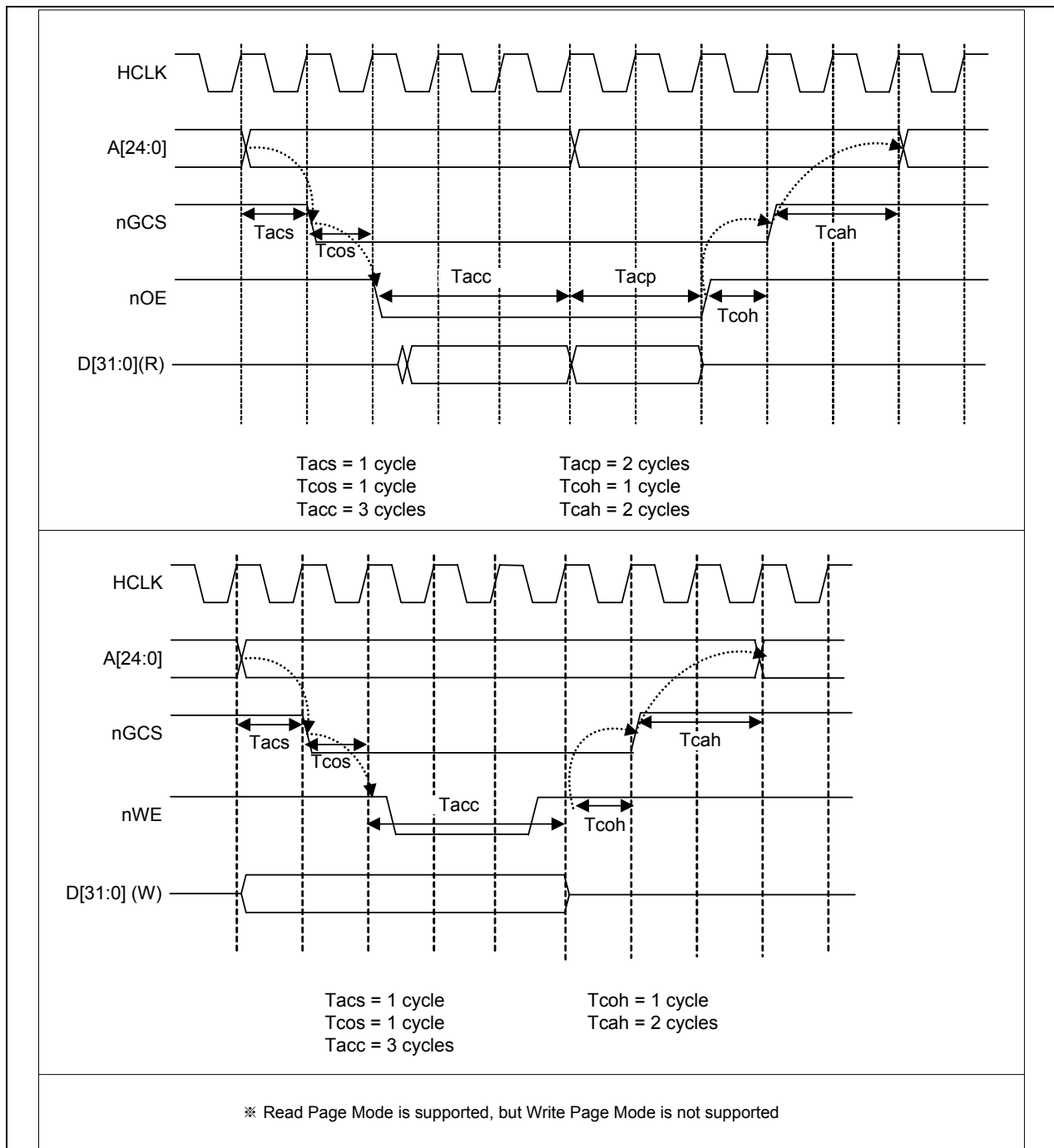
Figure 5-12. S3C2440A nGCS Timing Diagram
