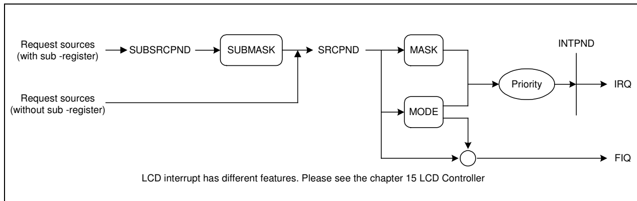
Figure 14-1. Interrupt Process Diagram
