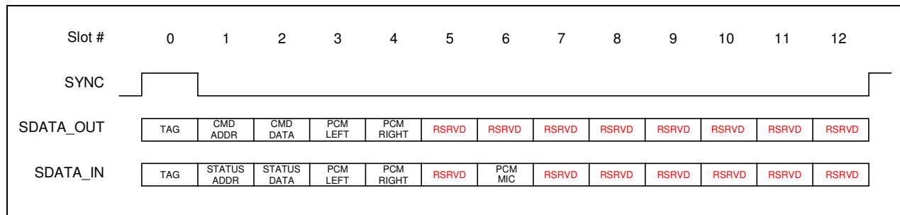
Figure 24-4. Bi-directional AC-link Frame with Slot Assignments
