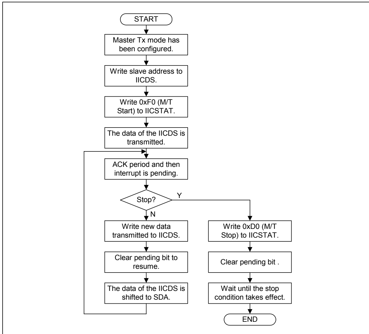
Figure 20-6. Operations for Master/Transmitter Mode
