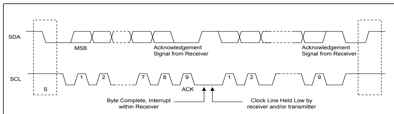
Figure 20-4. Data Transfer on the IIC-Bus
