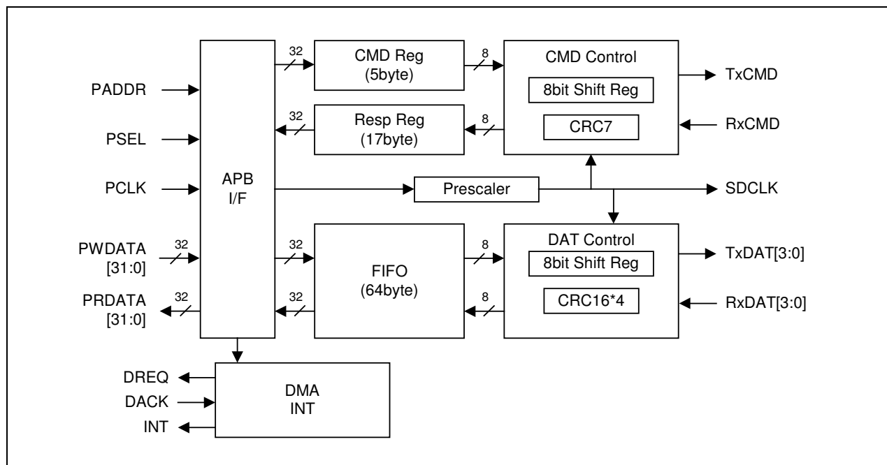
Figure 19-1. SD Interface block diagram
