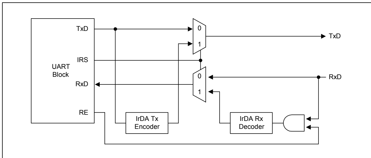
Figure 11-4. IrDA Function Block Diagram
