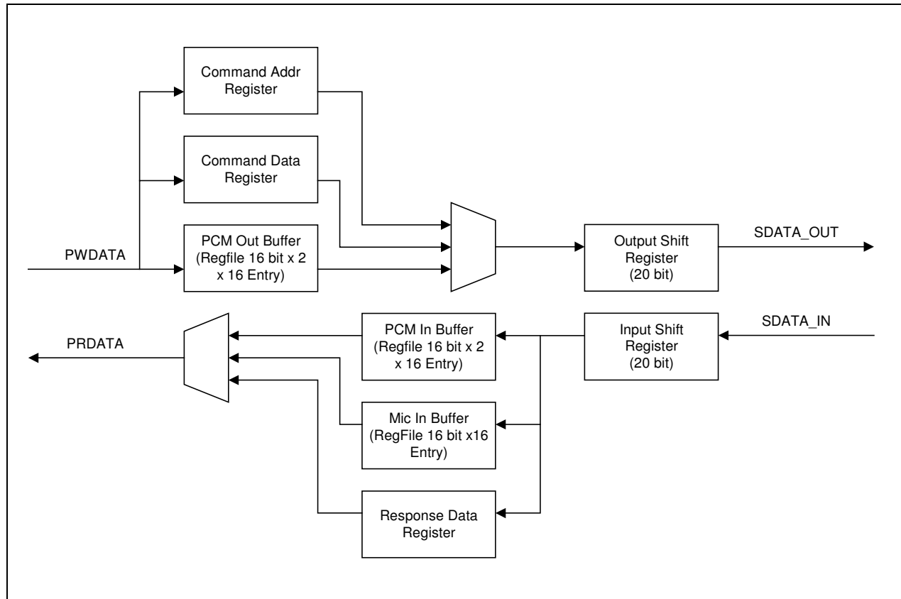
Figure 24-2. Internal Data Path
