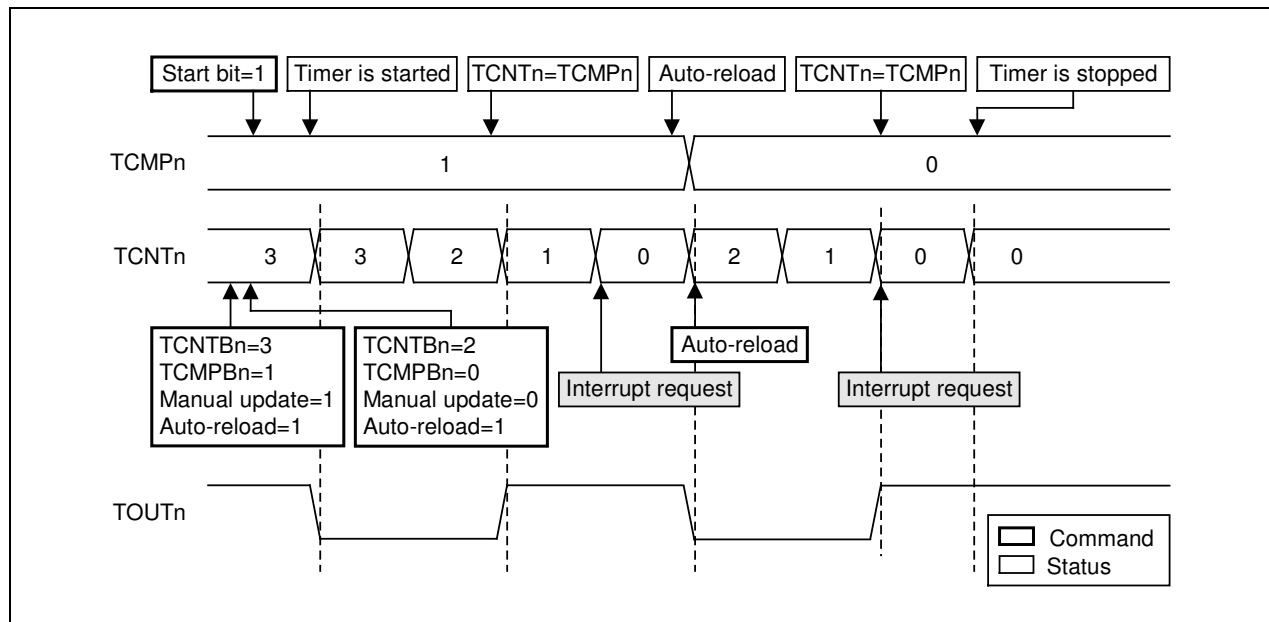
Figure 10-2. Timer Operations
