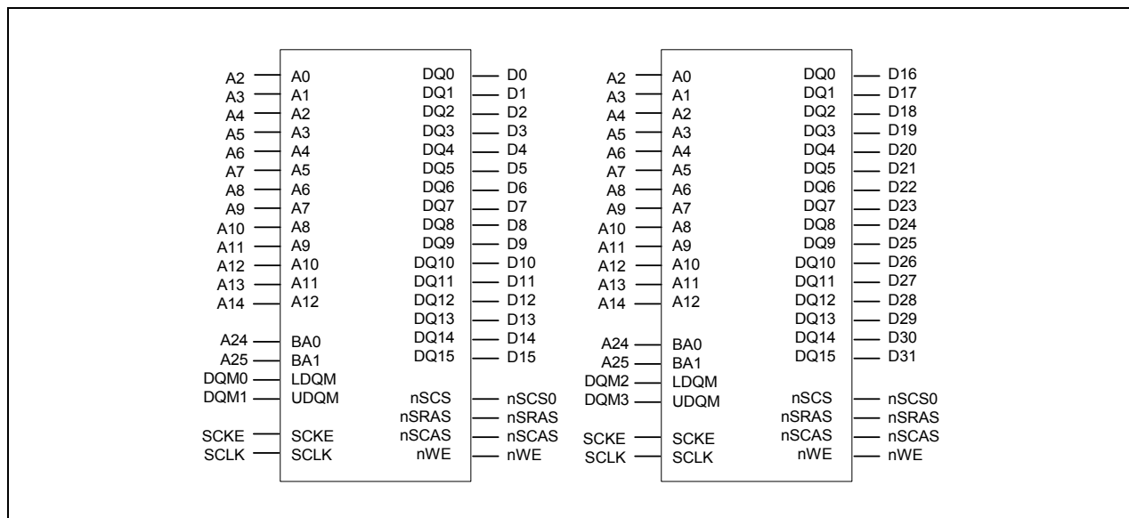
Figure 5-11. Memory Interface with 16-bit SDRAM (4Mx16x4Bank * 2ea)
