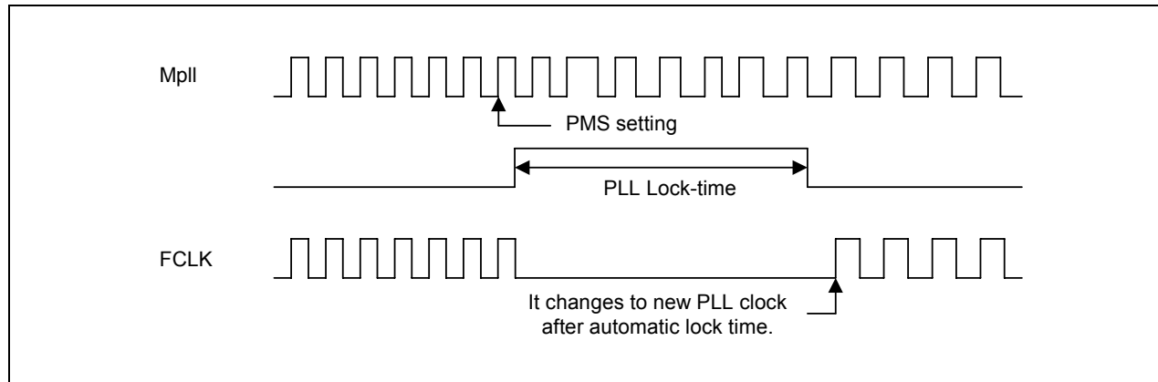
Figure 7-5. Changing Slow Clock by Setting PMS Value
