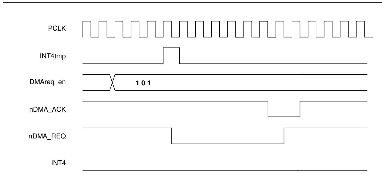
Figure 10-8. Timer4 DMA Mode Operation
