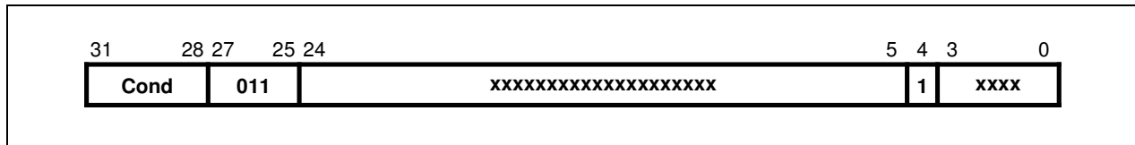
Figure 3-28. Undefined Instruction
