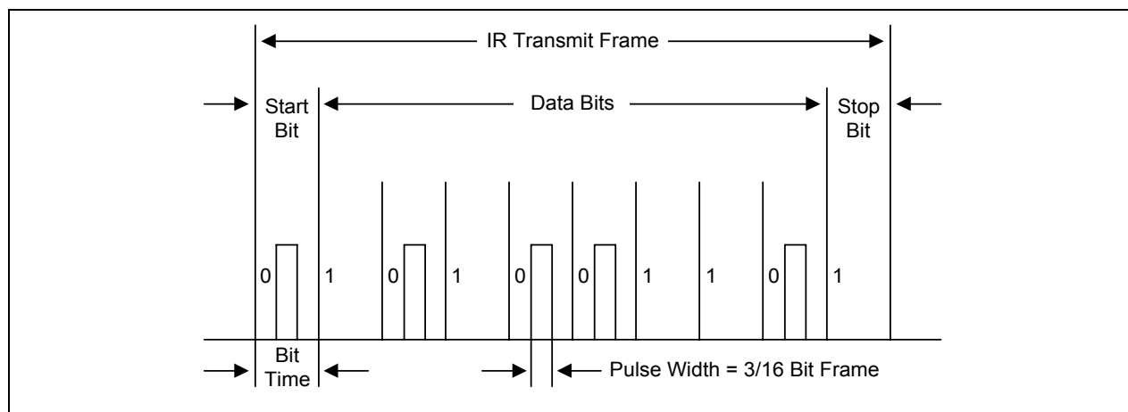
Figure 11-6. Infrared Transmit Mode Frame Timing Diagram
