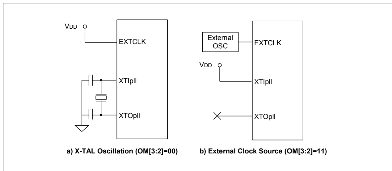
Figure 7-3. Main Oscillator Circuit Examples
