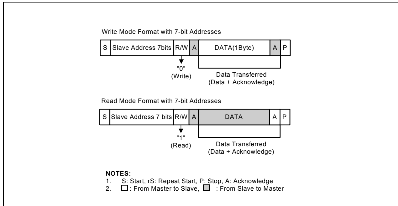
Figure 20-3. IIC-Bus Interface Data Format
