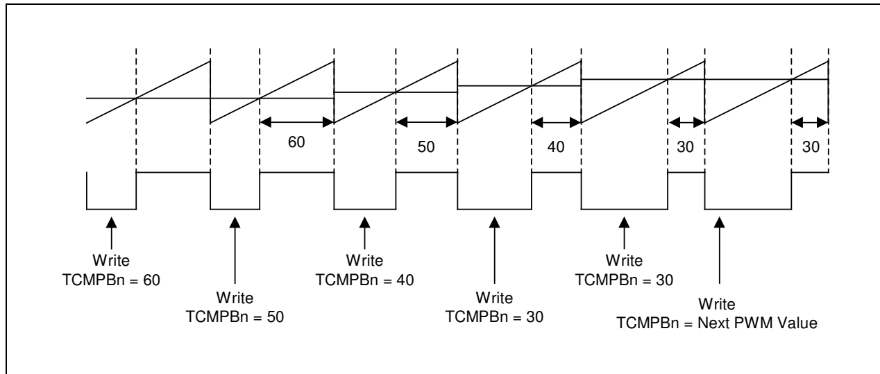
Figure 10-5. Example of PWM
