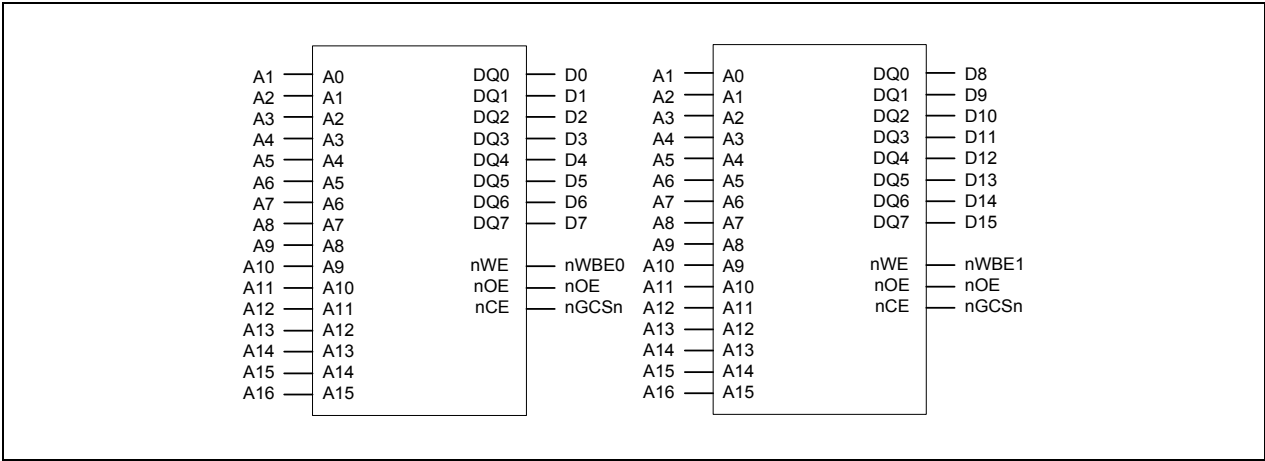
Figure 5-5. Memory Interface with 8-bit ROM x 2
