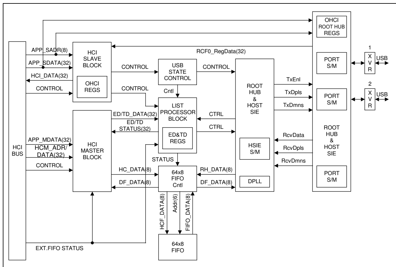
Figure 12-1. USB Host Controller Block Diagram
