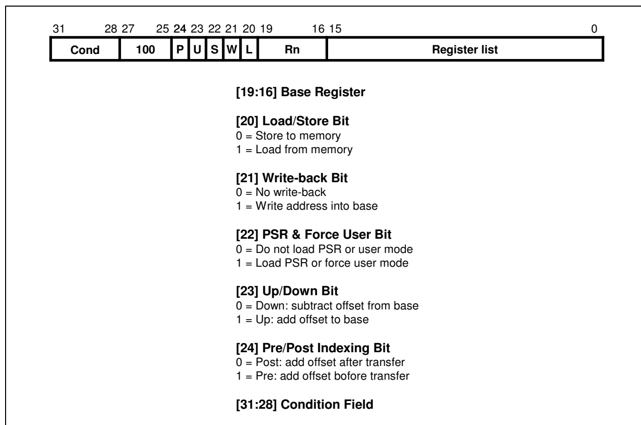
Figure 3-18. Block Data Transfer Instructions
