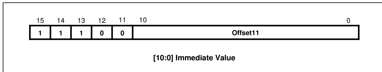
Figure 4-19. Format 18
