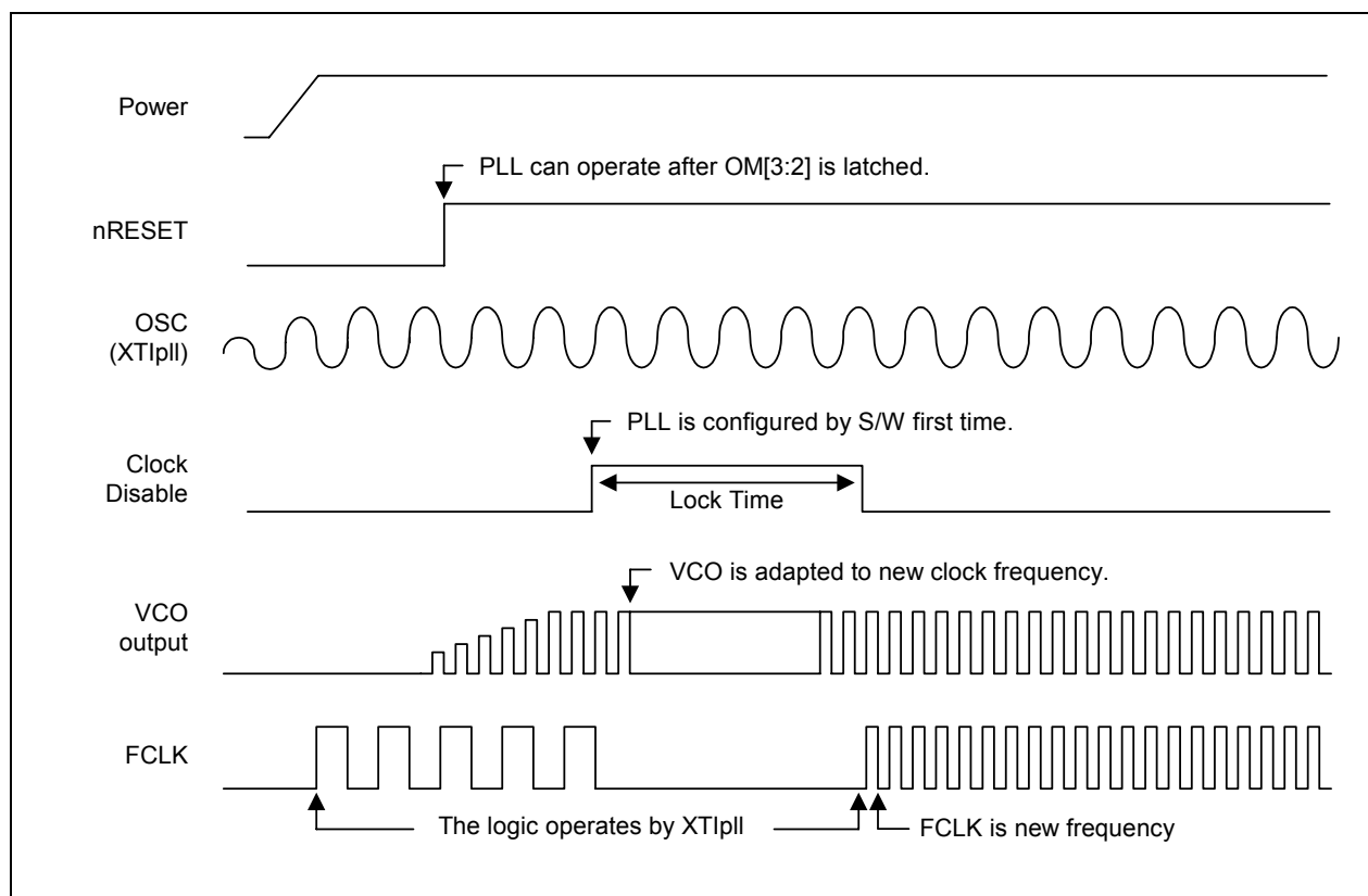
Figure 7-4. Power-On Reset Sequence (when the external clock source is a crystal oscillator)
