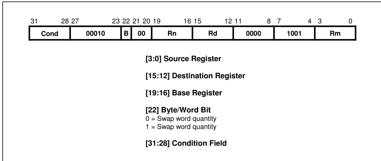
Figure 3-23. Swap Instruction
