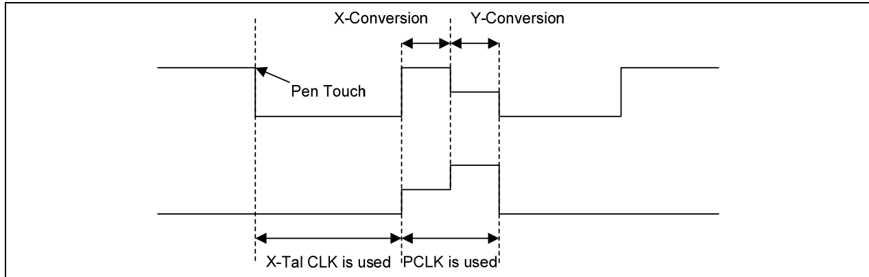
Figure 16-2. ADC and Touch Screen Operation signal
