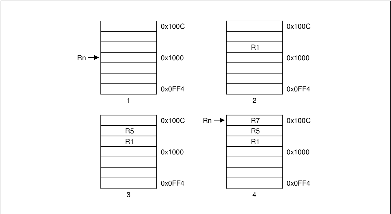
Figure 3-20. Pre-Increment Addressing
