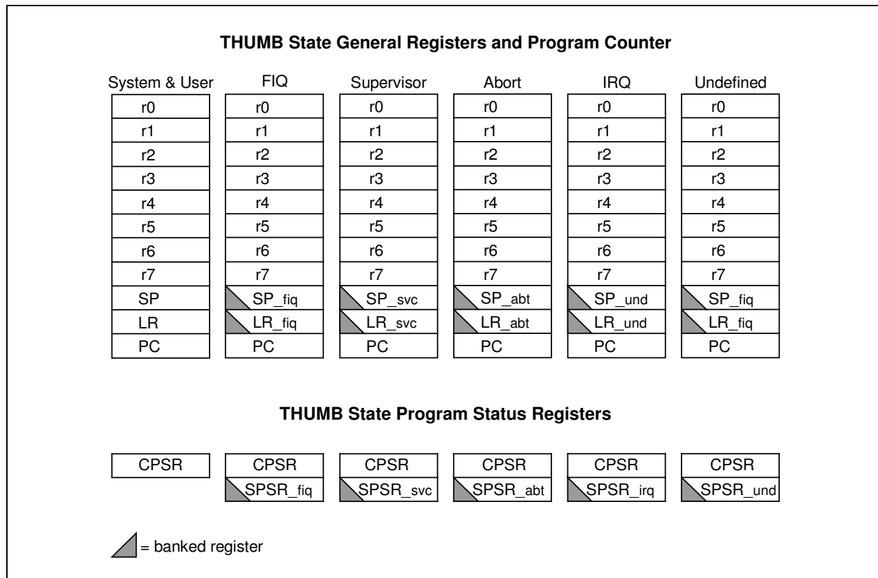
Figure 2-4. Register Organization in THUMB state
