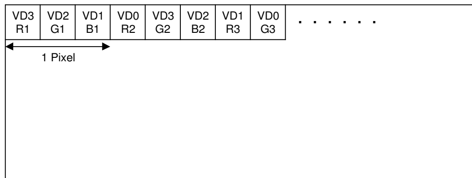
4-bit Single Scan Display
