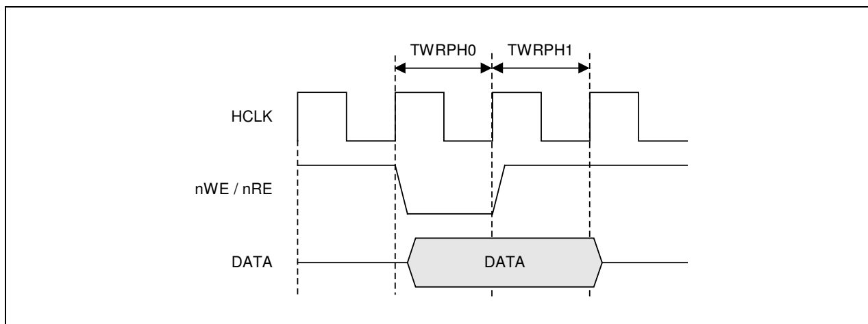
Figure 6-4. nWE &amp; nRE Timing (TWRPH0=0, TWRPH1=0)
