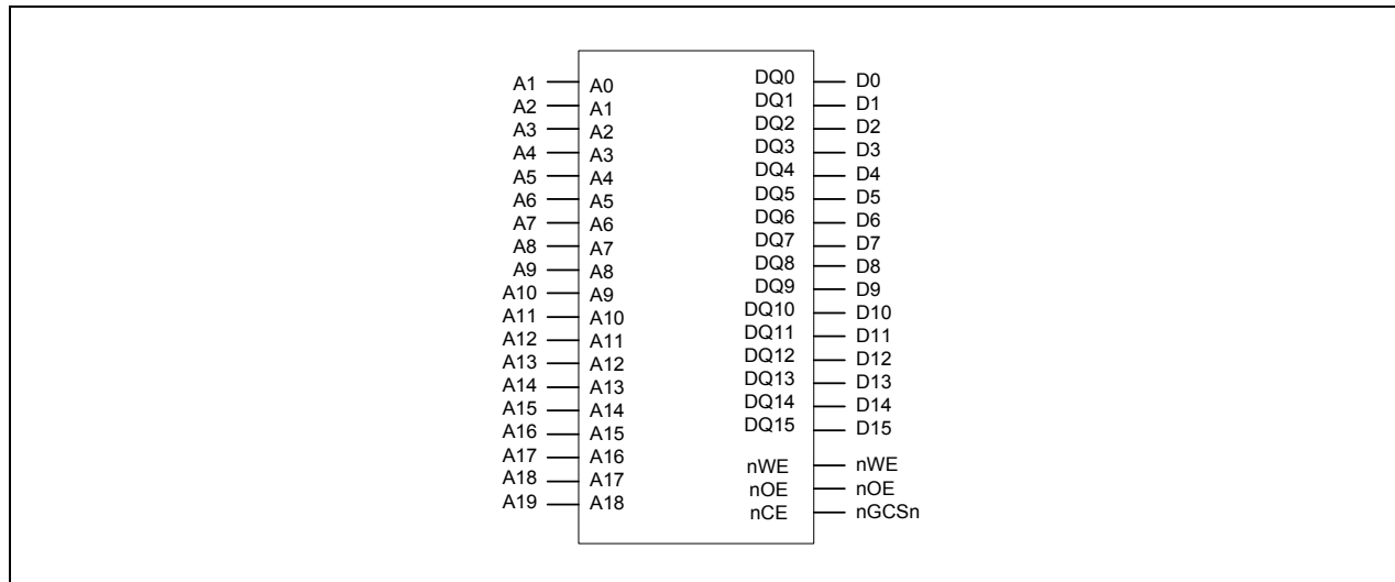
Figure 5-7. Memory Interface with 16-bit ROM
