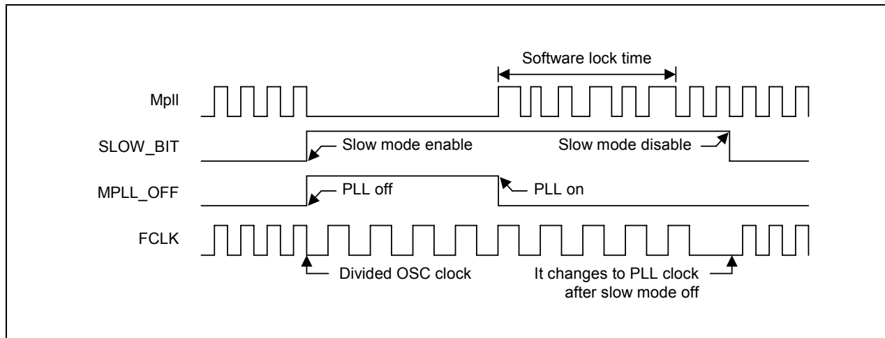
Figure 7-10. Issuing Exit_from_Slow_mode Command After Lock Time
