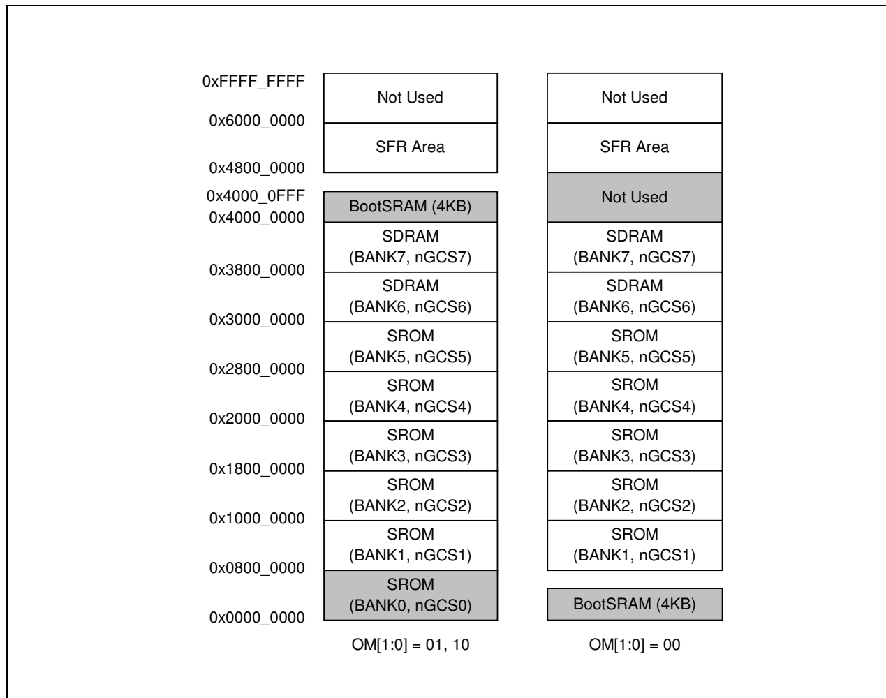
Figure 6-5. NAND Flash Memory Mapping
