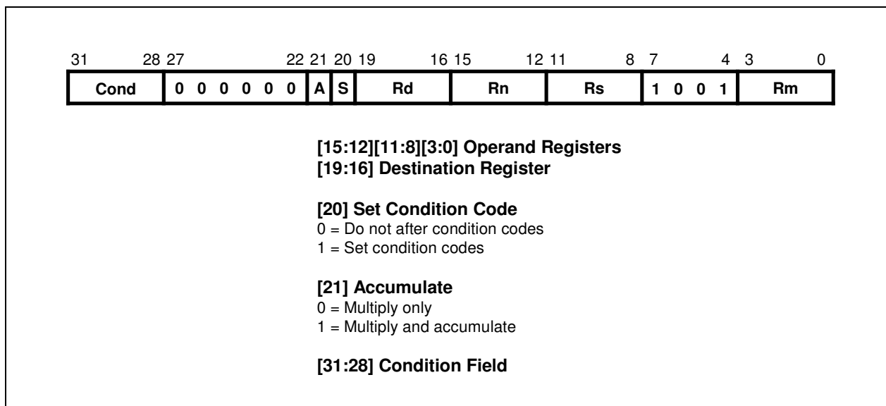
Figure 3-12. Multiply Instructions
