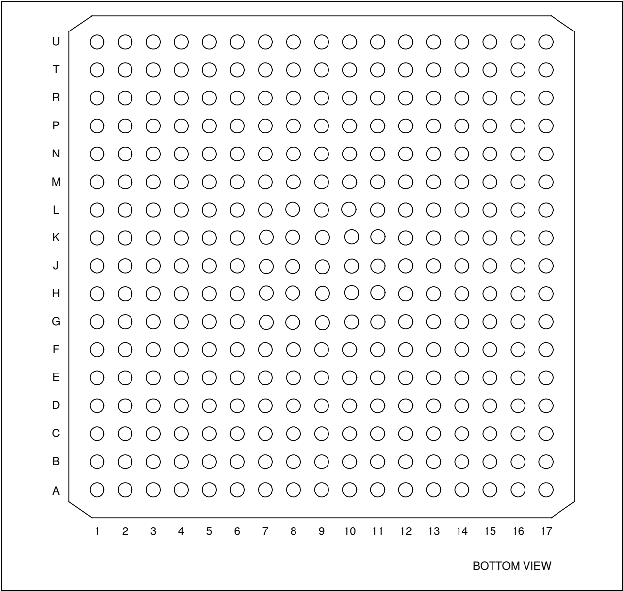
Figure 1-2. S3C2440A Pin Assignments (289-FBGA)
