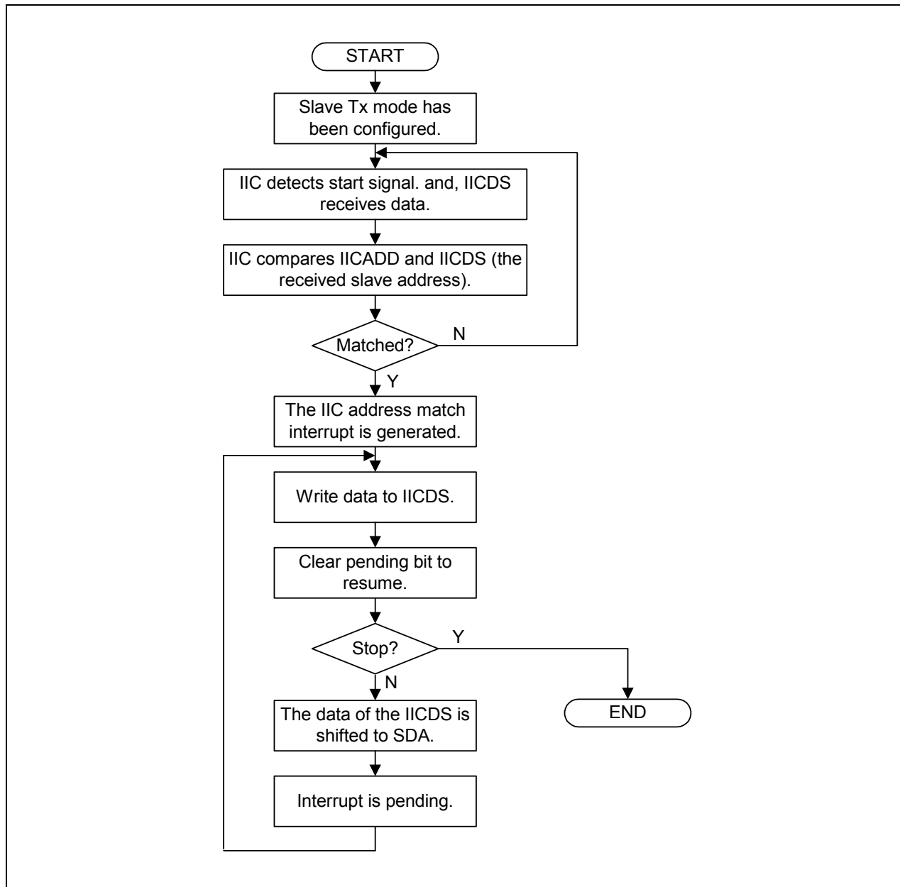
Figure 20-8. Operations for Slave/Transmitter Mode
