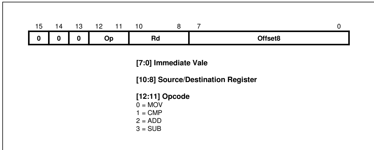
Figure 4-4. Format 3
