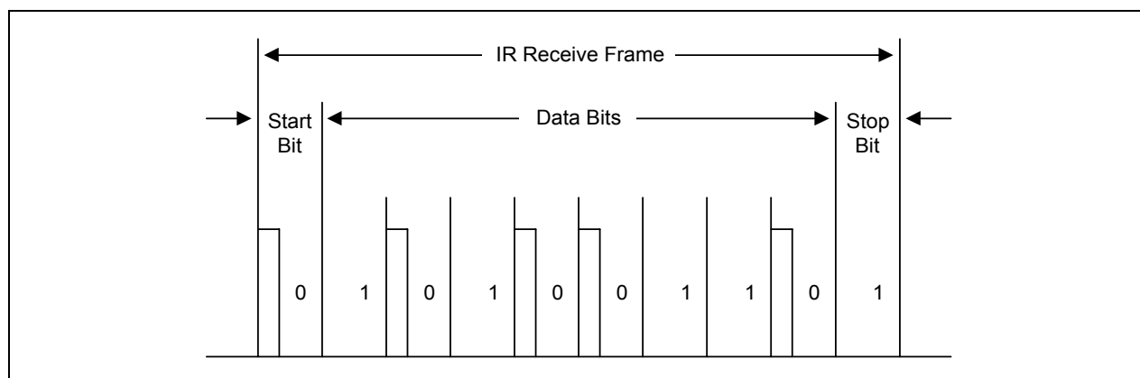
Figure 11-7. Infrared Receive Mode Frame Timing Diagram
