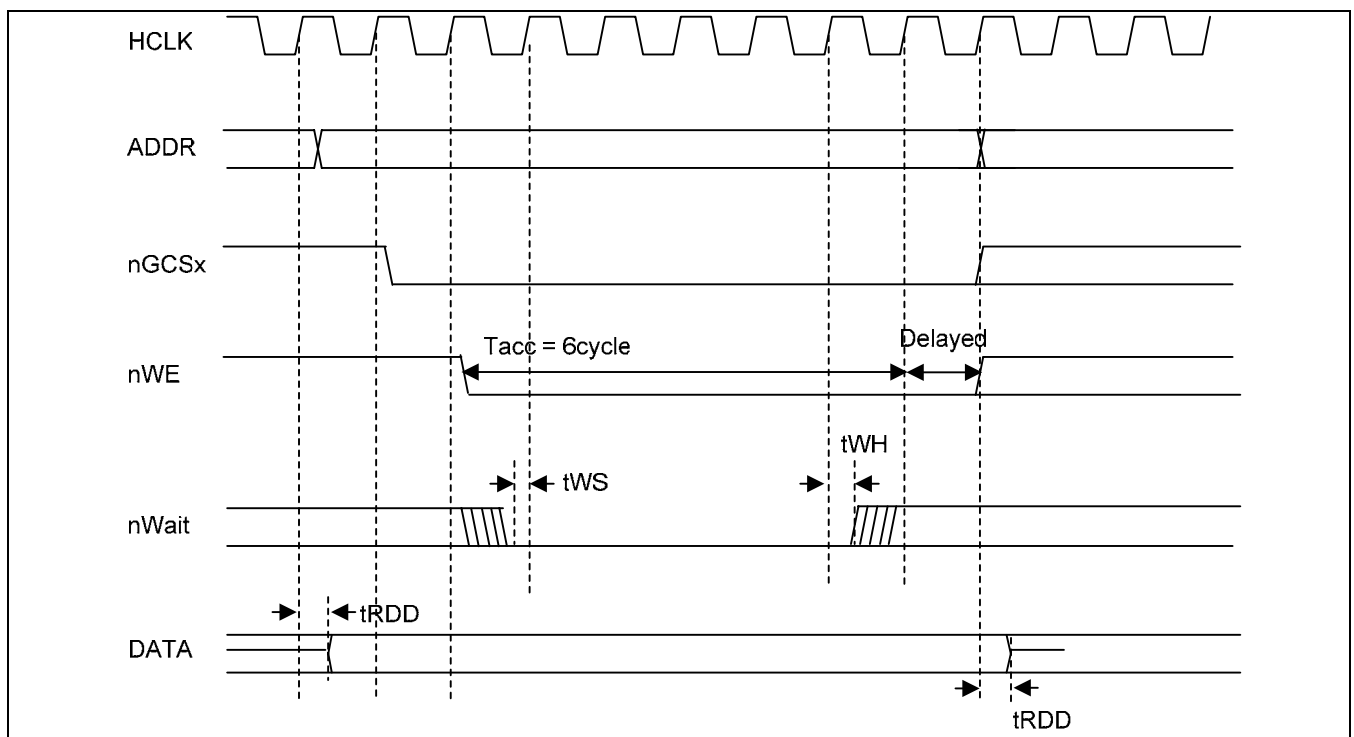
Figure 27-17. External nWAIT WRITE Timing Diagram (Tacs=1, Tcos=1, Tacc=4(6-cycle), Toch=0, Tcah=0, PMC=0, ST=0)
