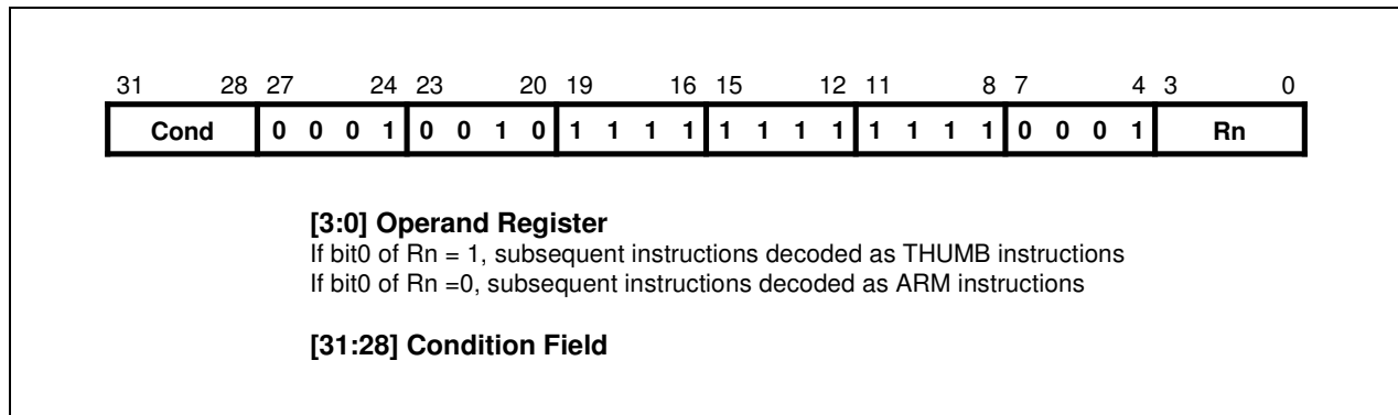
Figure 3-2. Branch and Exchange Instructions
