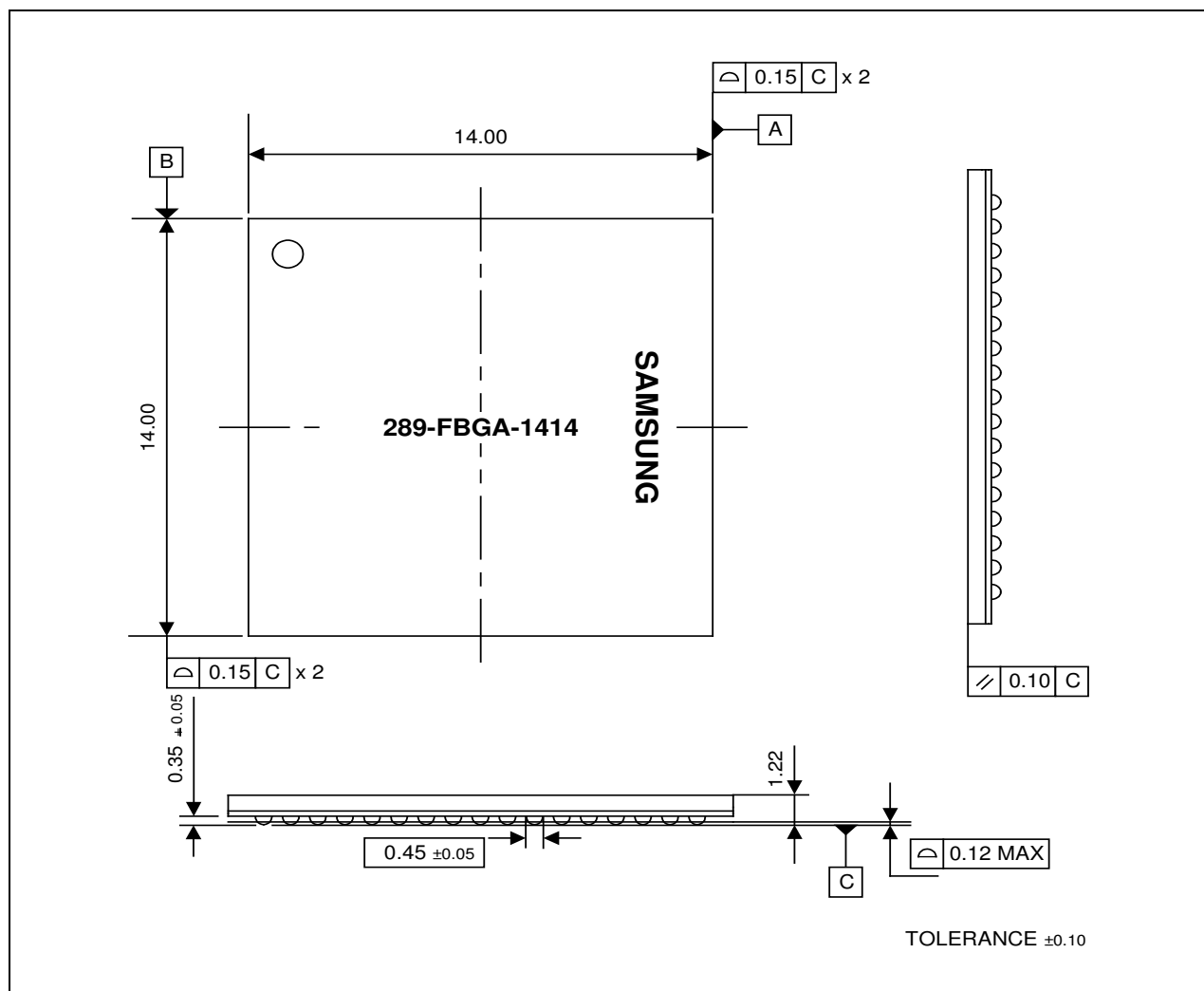
Figure 26-1. 289-FBGA-1414 Package Dimension 1 (Top View)
