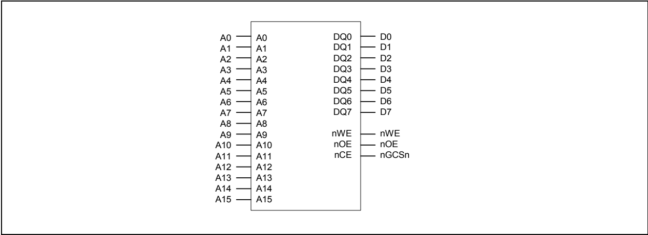
Figure 5-4. Memory Interface with 8-bit ROM
