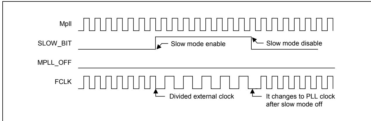
Figure 7-9. Issuing Exit_from_Slow_mode Command in PLL on State
