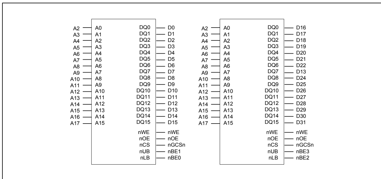
Figure 5-9. Memory Interface with 16-bit SRAM x 2
