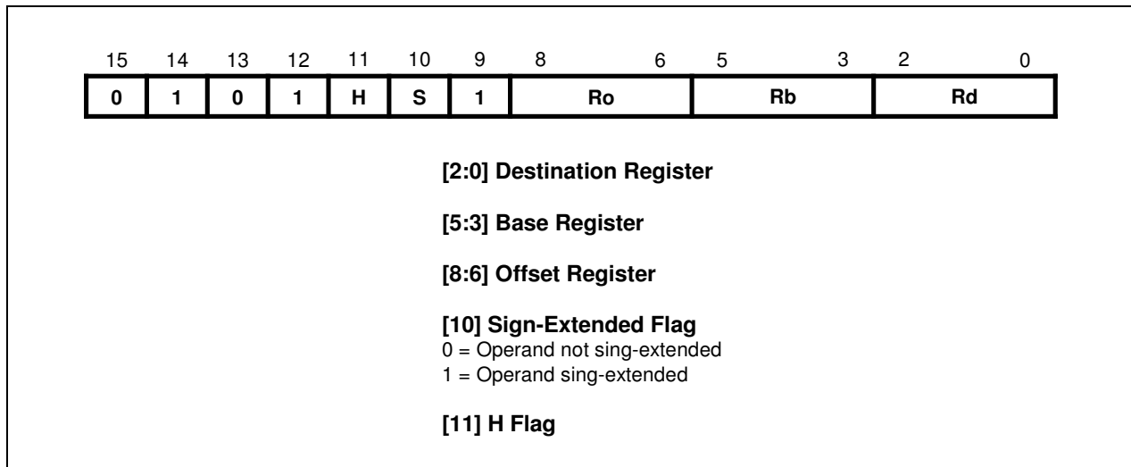
Figure 4-9. Format 8
