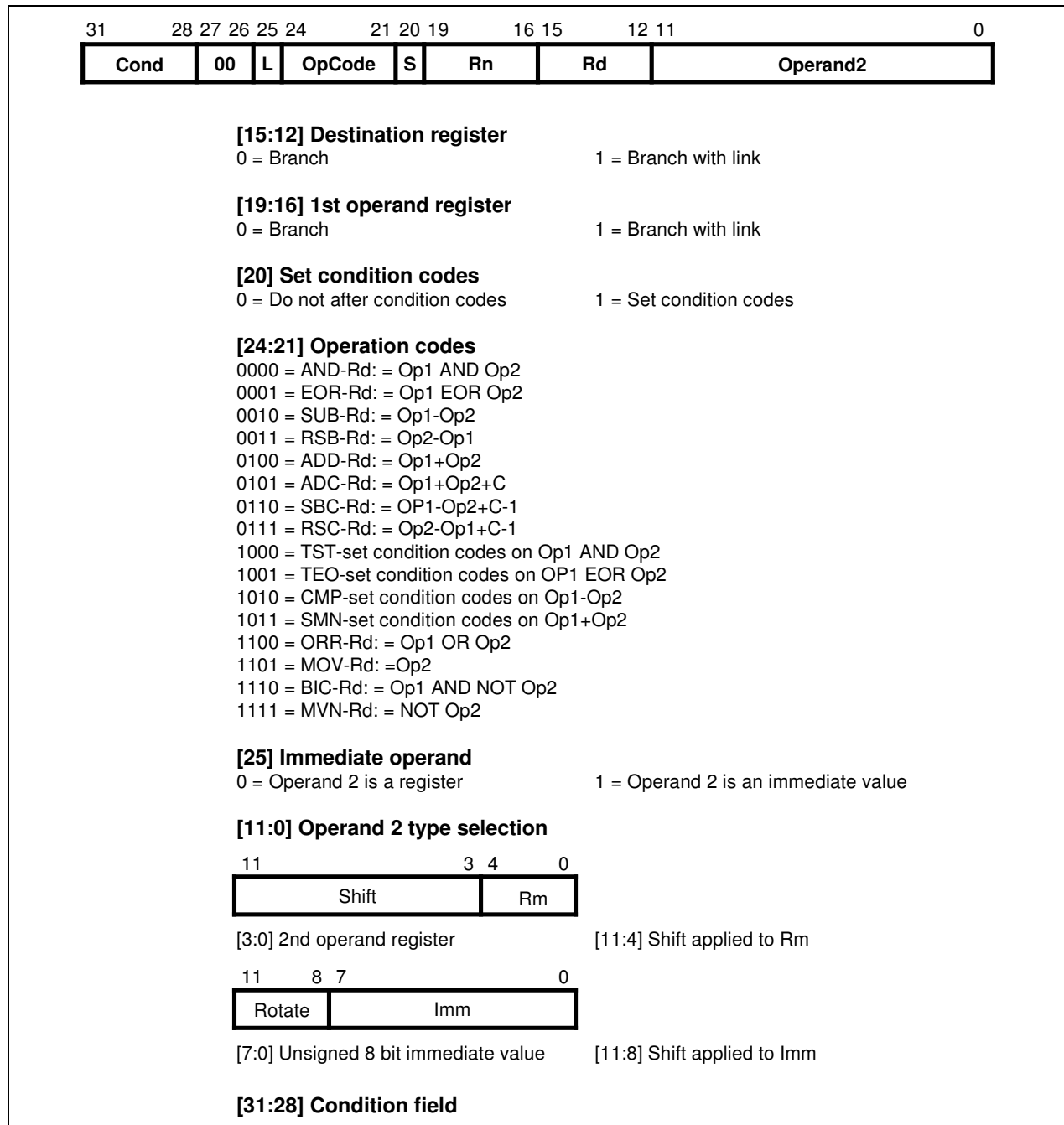
Figure 3-4. Data Processing Instructions
