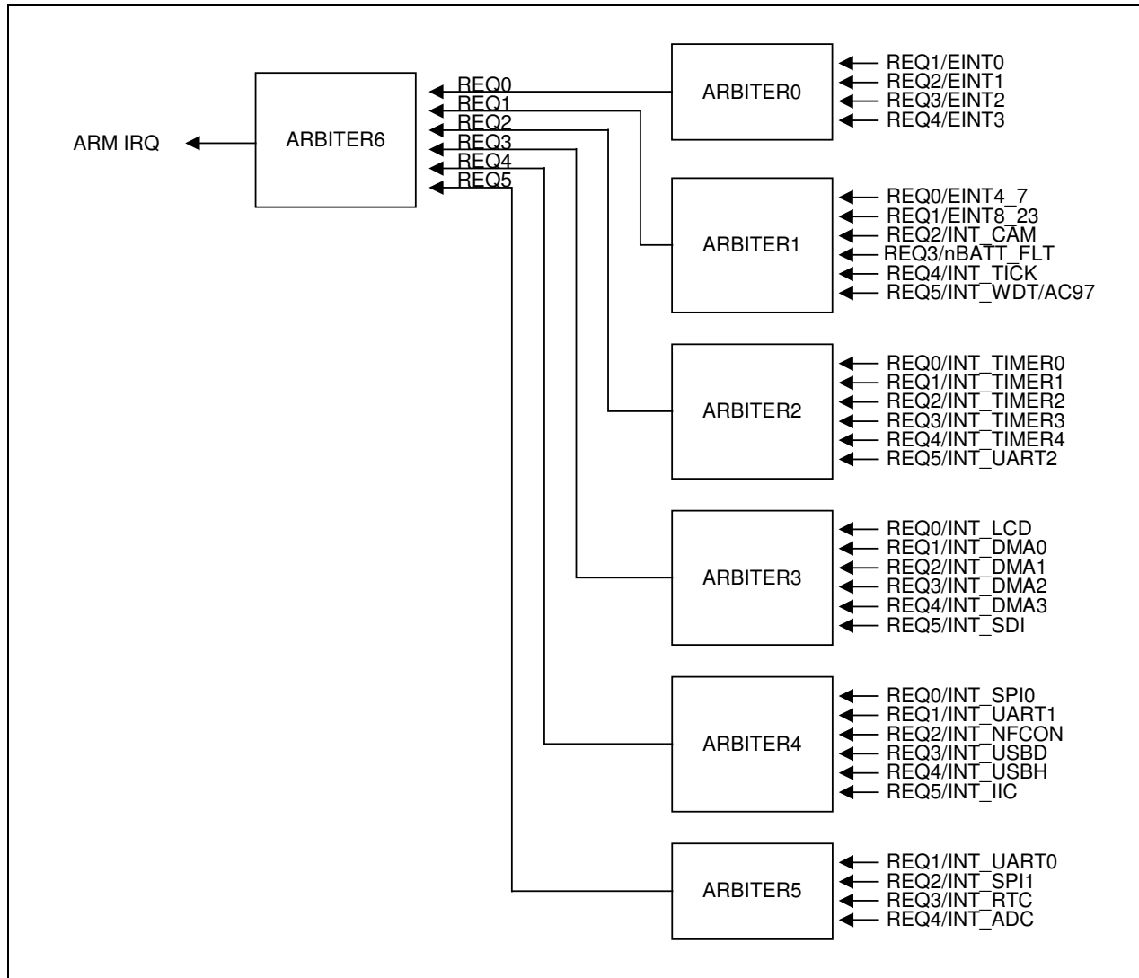
Figure 14-2. Priority Generating Block
