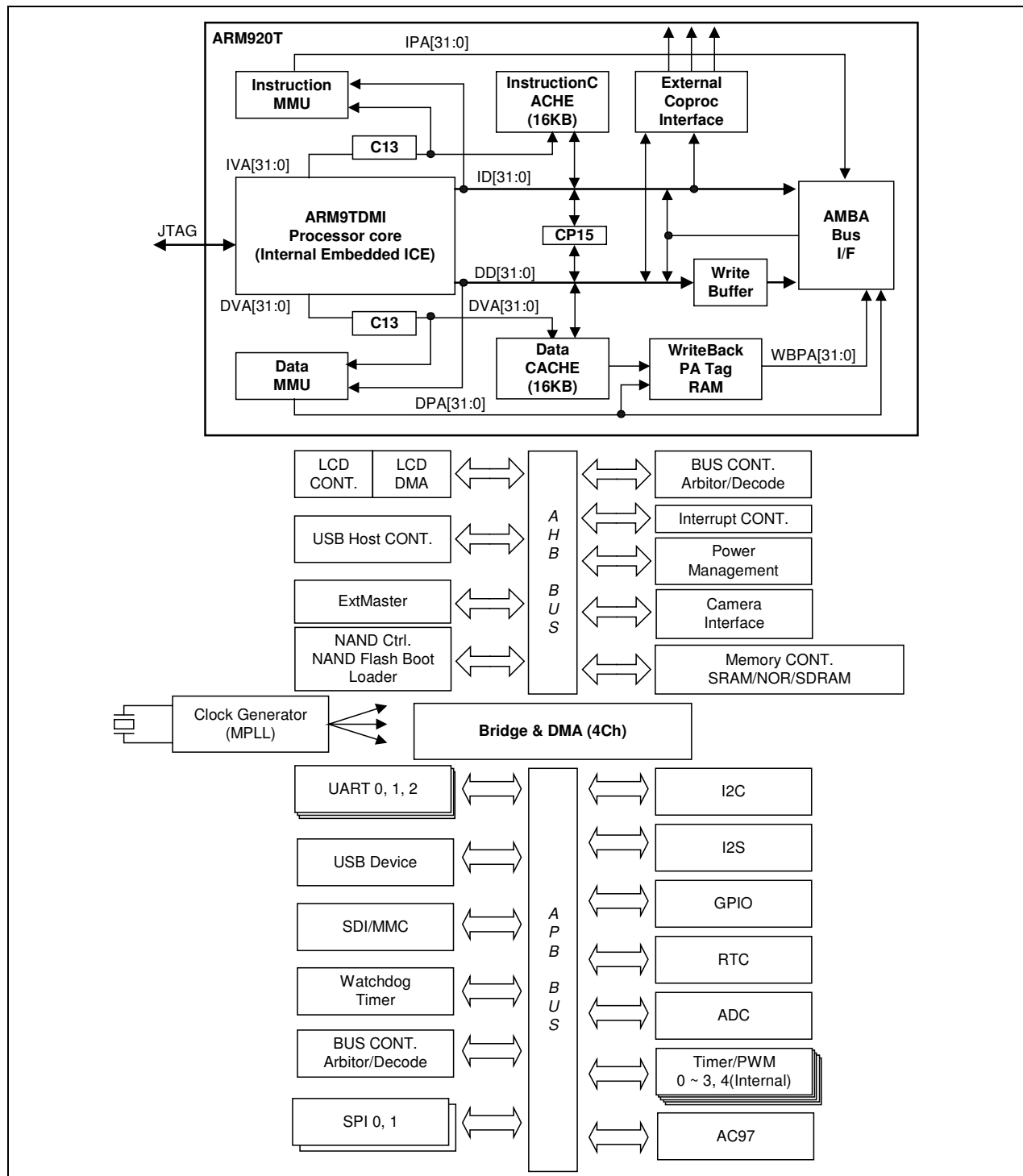
Figure 1-1. S3C2440A Block Diagram
