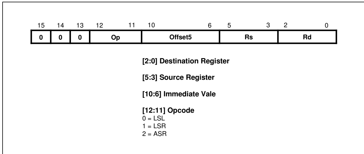
Figure 4-2. Format 1
