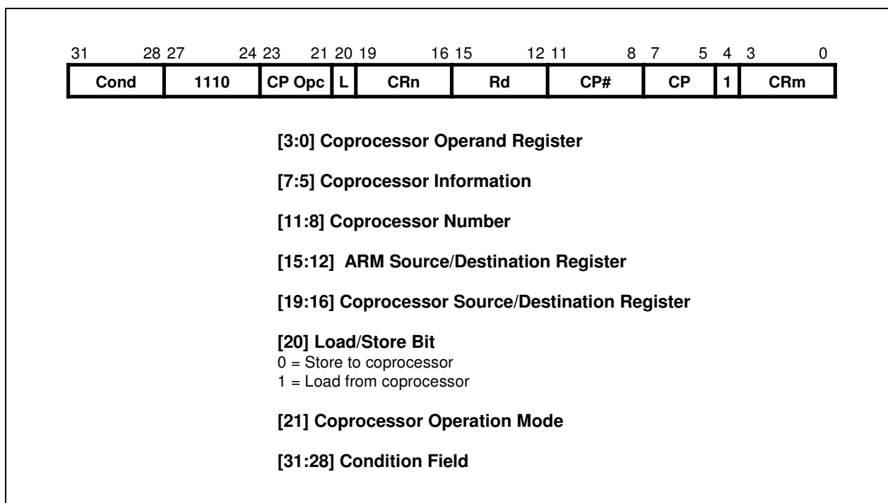
Figure 3-27. Coprocessor Register Transfer Instructions
