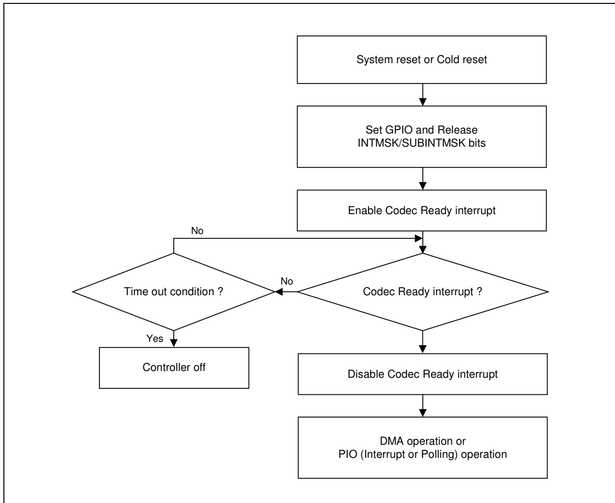
Figure 24-3. AC97 Operation Flow Chart
