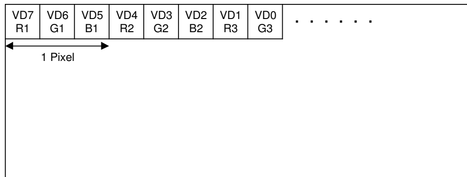
8-bit Single Scan Display
