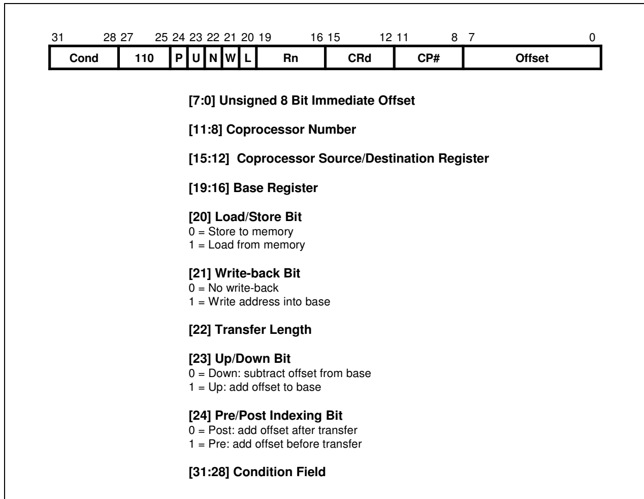
Figure 3-26. Coprocessor Data Transfer Instructions
