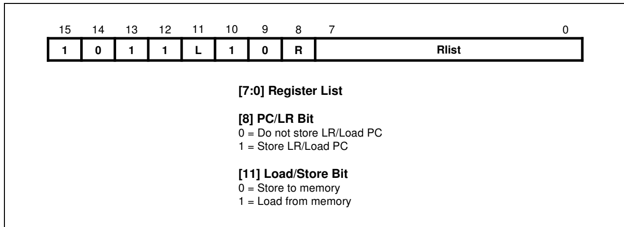
Figure 4-15. Format 14
