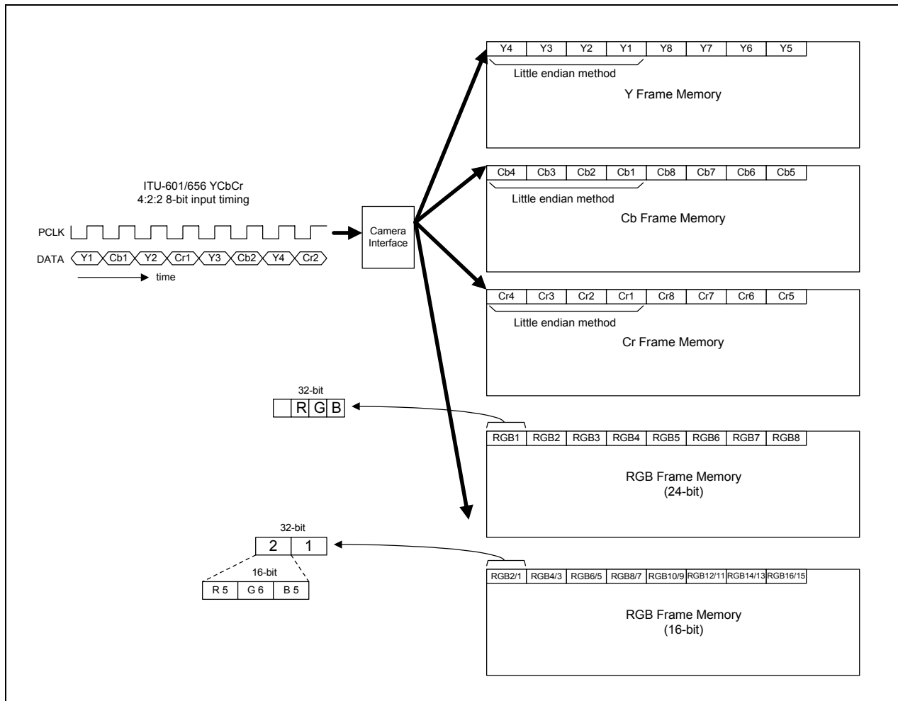
Figure 23-7. Memory Storing Style
