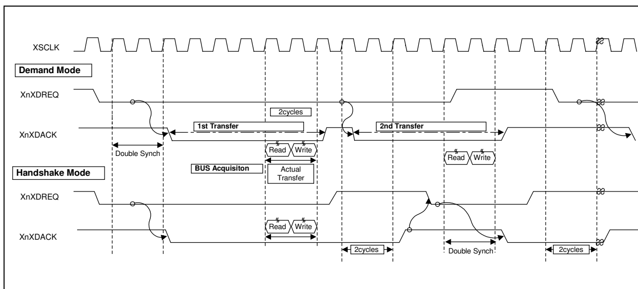
Figure 8-2. Demand/Handshake Mode Comparison
