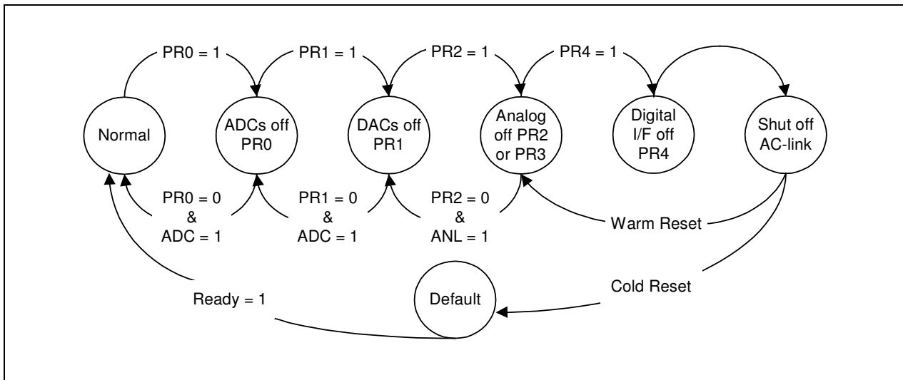
Figure 24-8. AC97 Power down/Power up Flow
