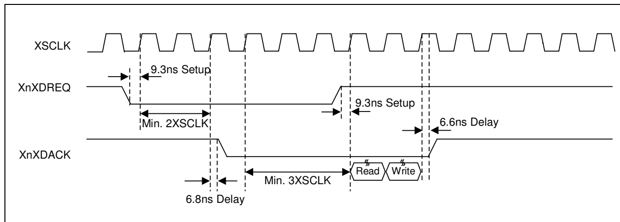
Figure 8-1. Basic DMA Timing Diagram
