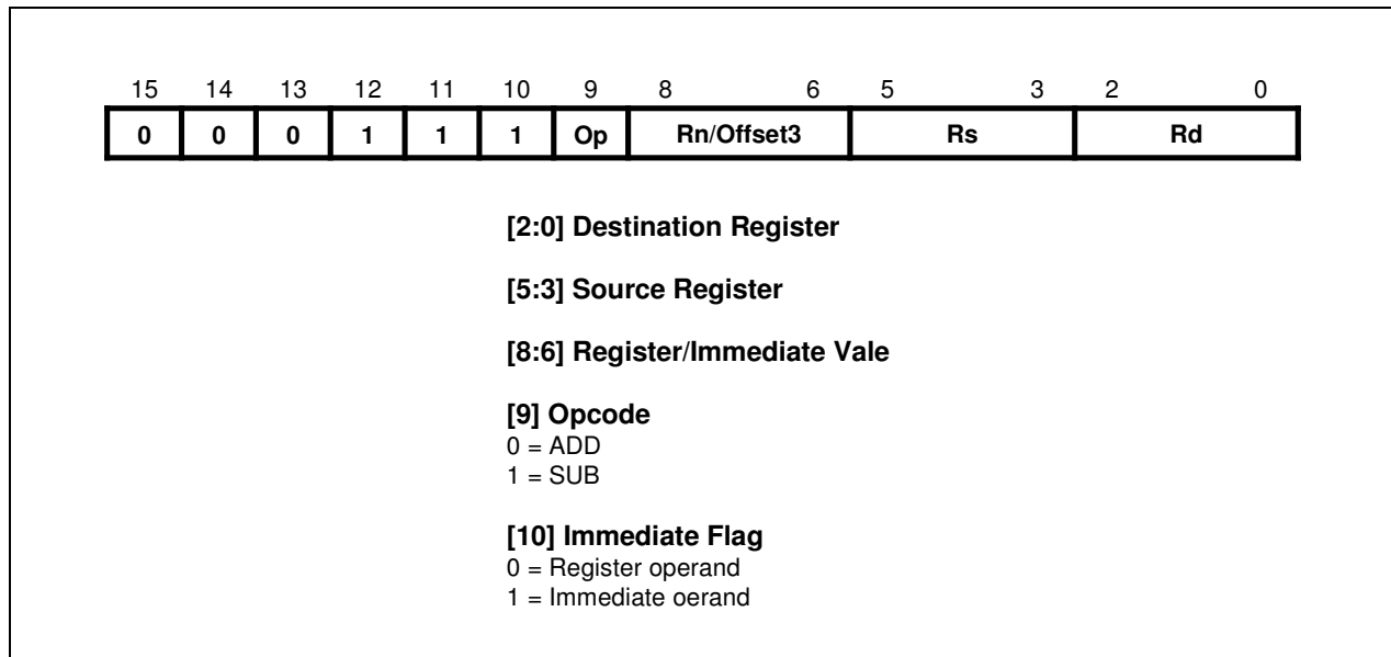
Figure 4-3. Format 2
