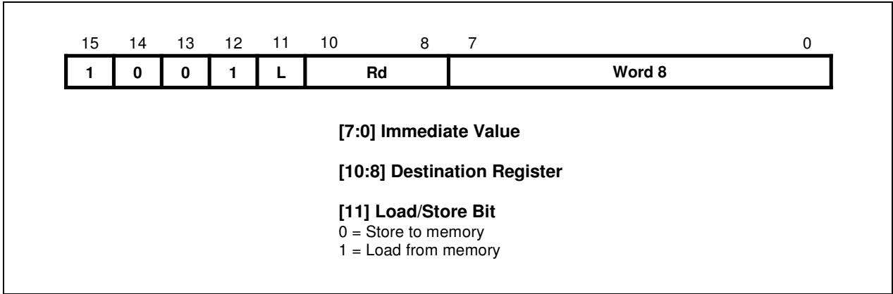
Figure 4-12. Format 11
