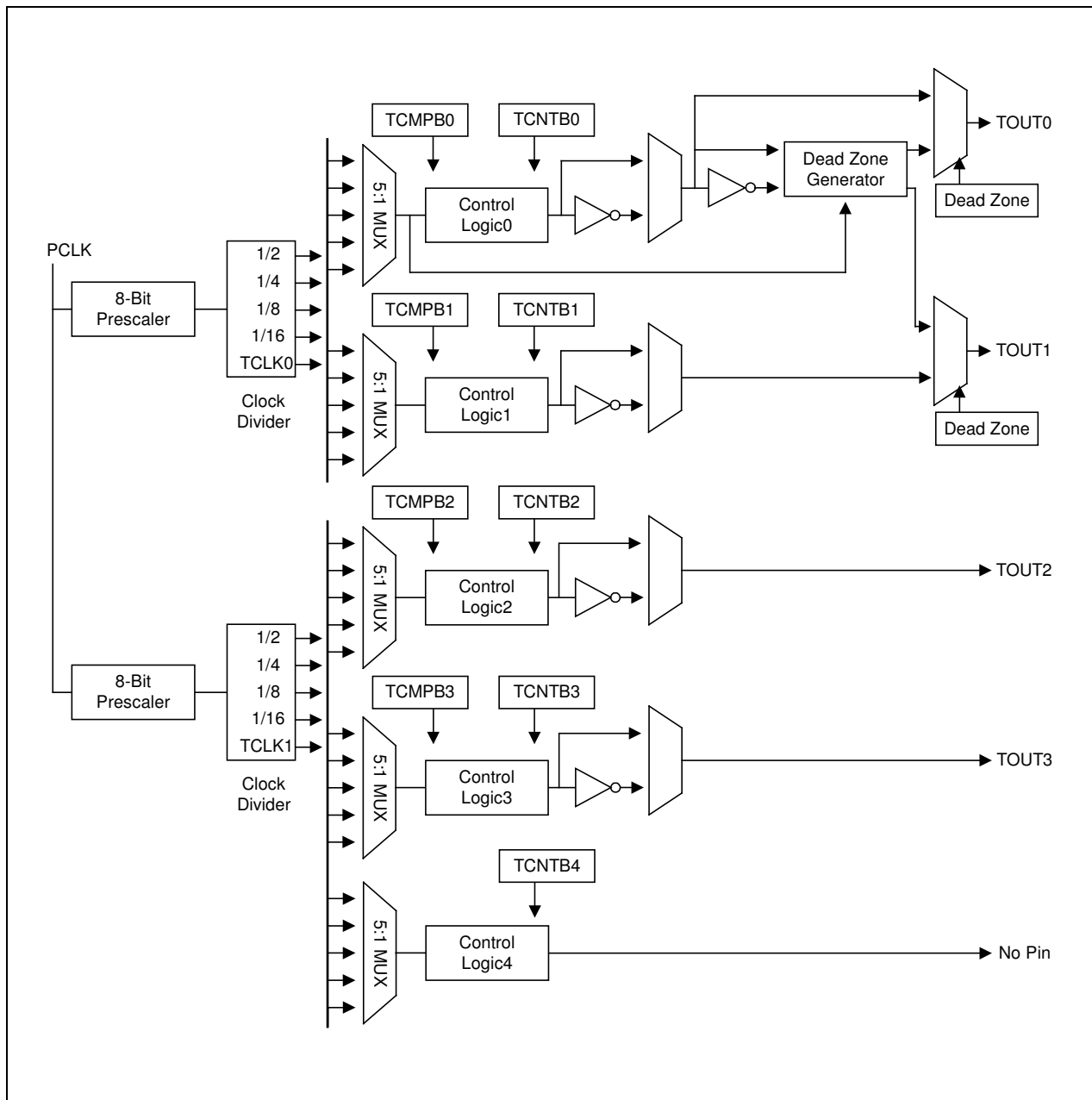
Figure 10-1. 16-bit PWM Timer Block Diagram
