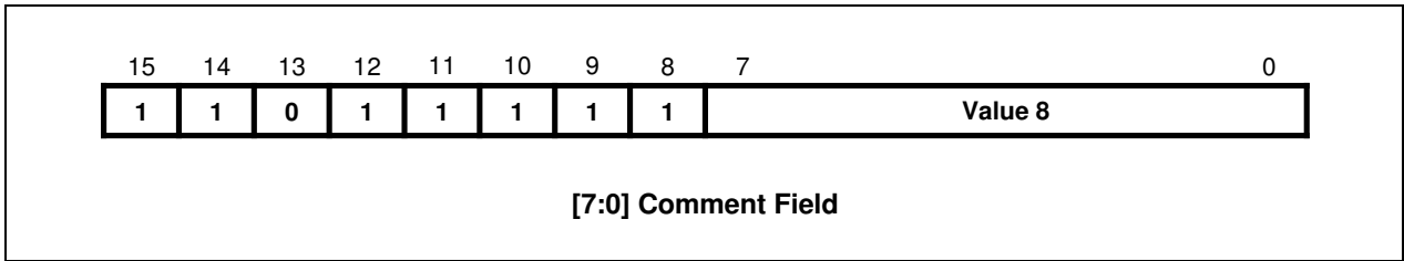
Figure 4-18. Format 17
