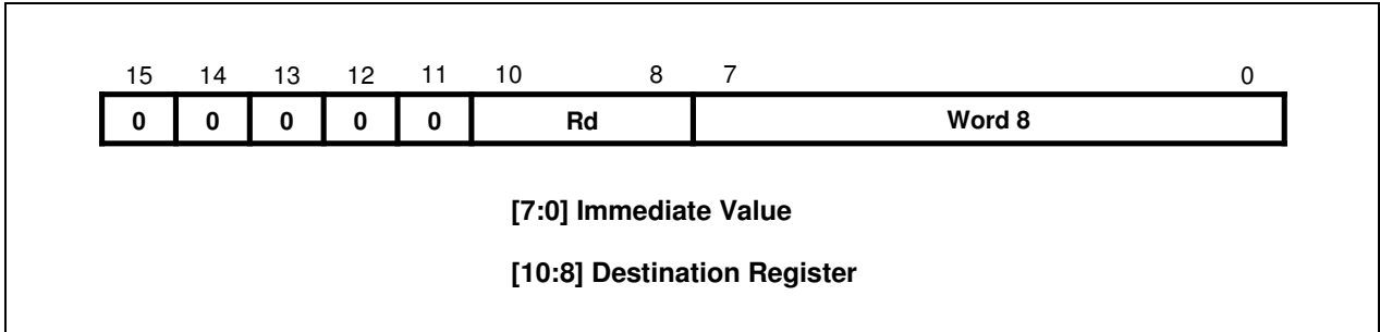
Figure 4-7. Format 6
