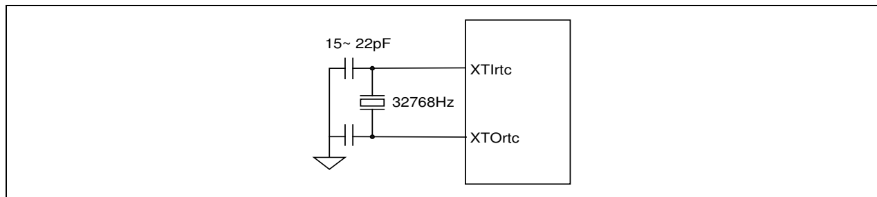
Figure 17-2. Main Oscillator Circuit Example
