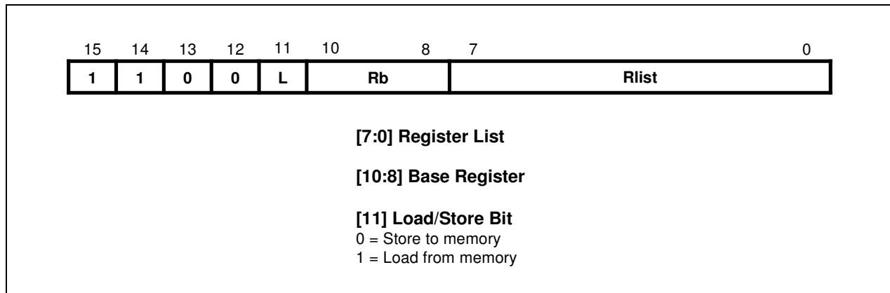
Figure 4-16. Format 15
