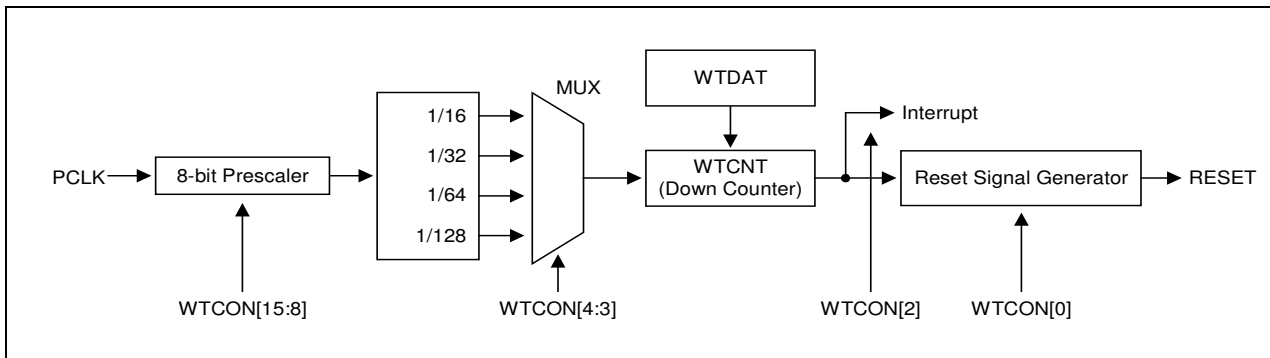
Figure 18-1. Watchdog Timer Block Diagram
