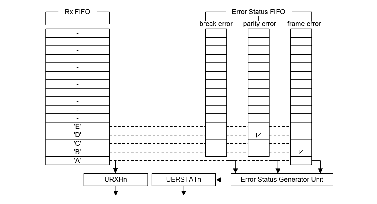
Figure 11-3. Example showing UART Receiving 5 Characters with 2 Errors
