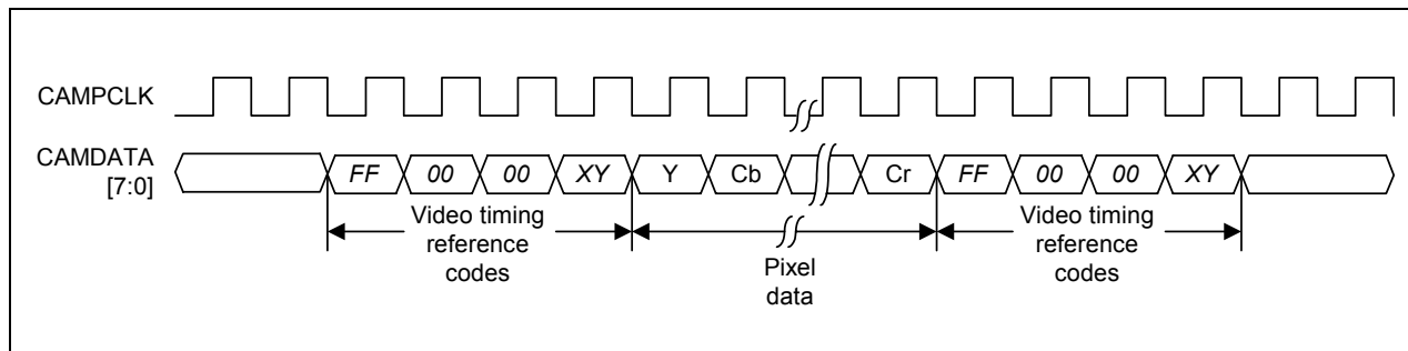
Figure 23-3. ITU-R BT 656 Input Timing Diagram
