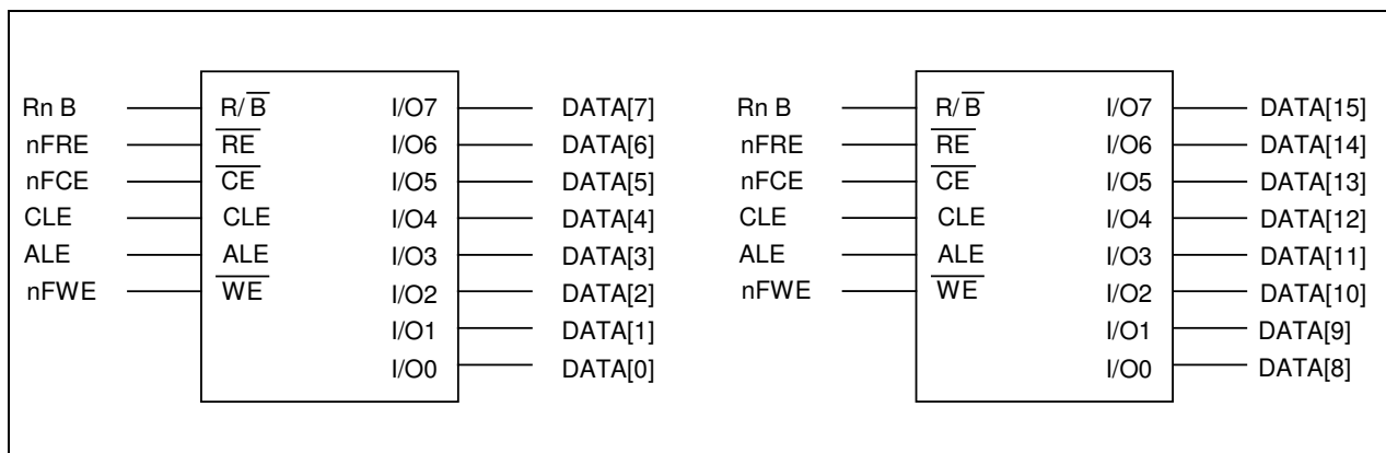
Figure 6-7. Two 8-bit NAND Flash Memory Interface
