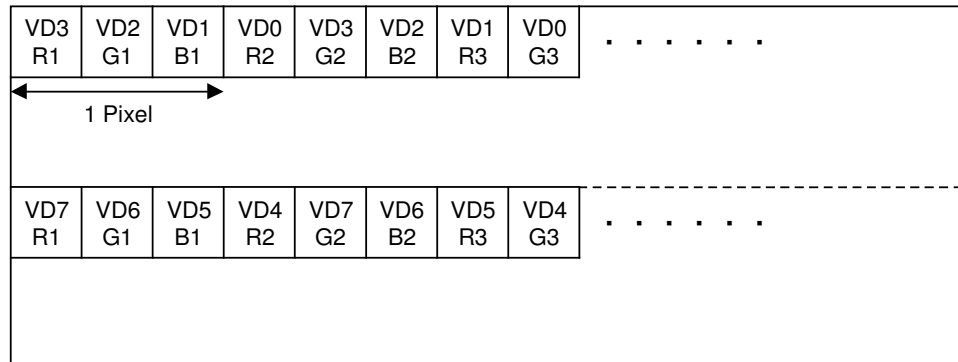
4-bit Dual Scan Display
