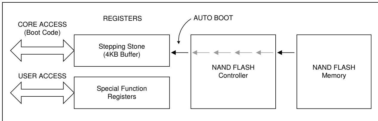
Figure 6-2. NAND Flash Controller Boot Loader Block Diagram
