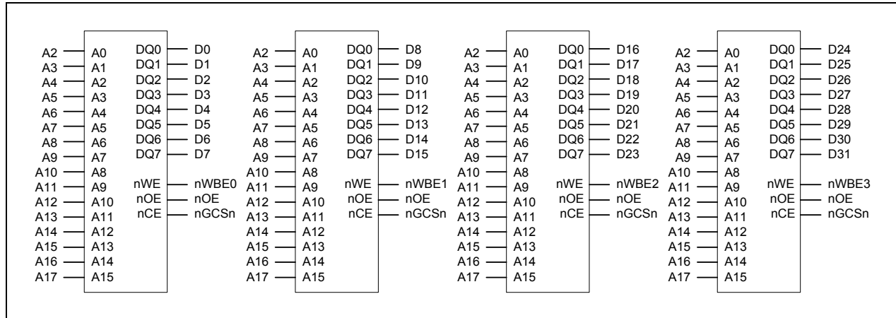
Figure 5-6. Memory Interface with 8-bit ROM x 4
