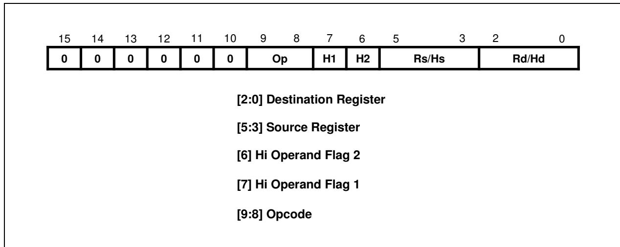
Figure 4-6. Format 5
