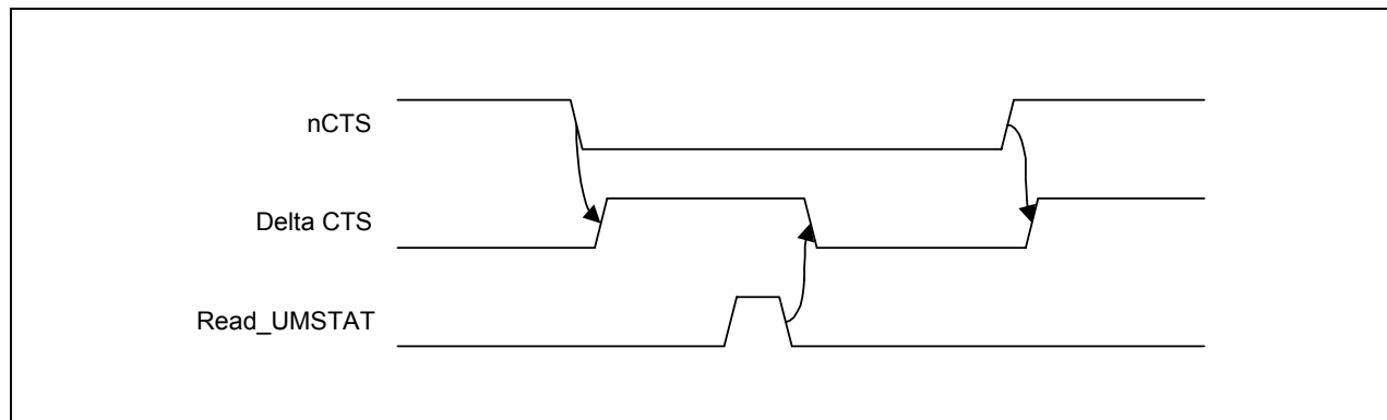
Figure 11-8. nCTS and Delta CTS Timing Diagram
