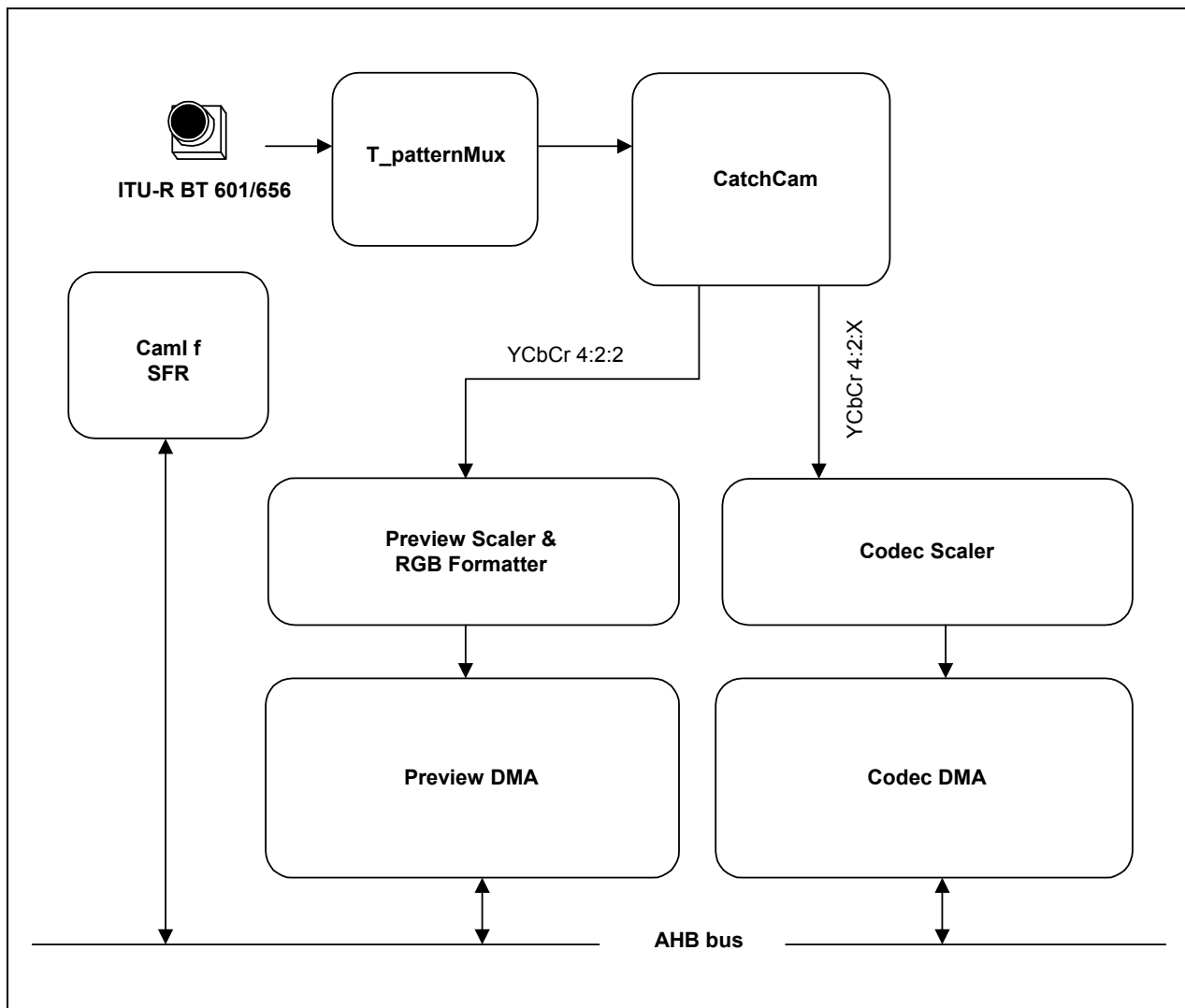
Figure 23-1. CAMIF Overview
