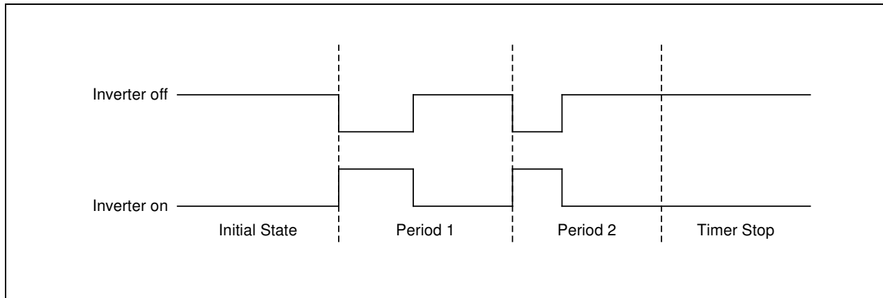
Figure 10-6. Inverter On/Off
