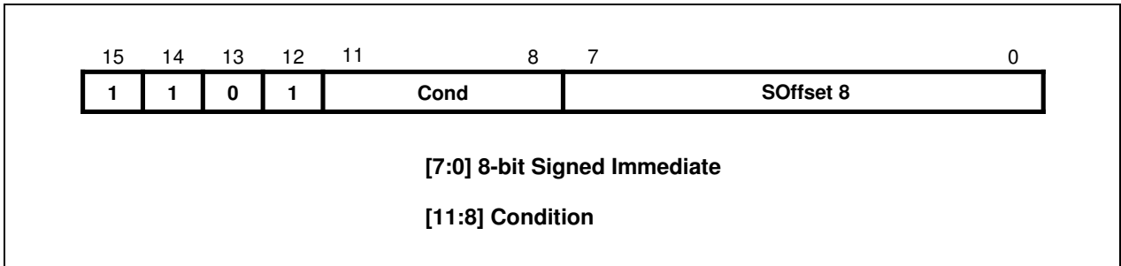
Figure 4-17. Format 16
