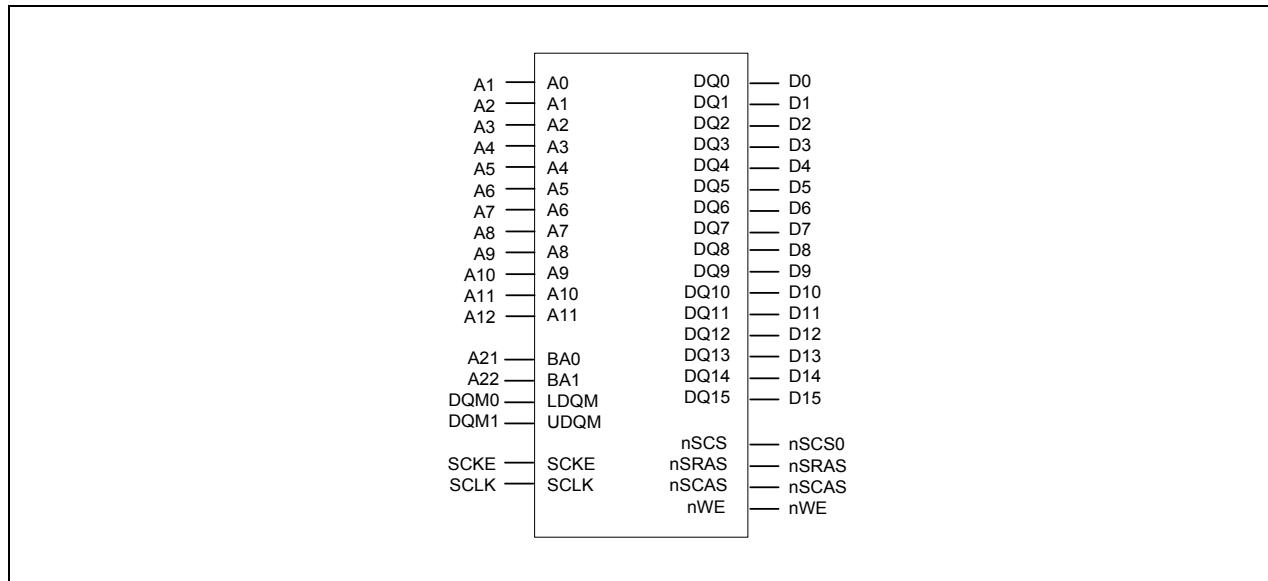
Figure 5-10. Memory Interface with 16-bit SDRAM (4Mx16, 4banks)
