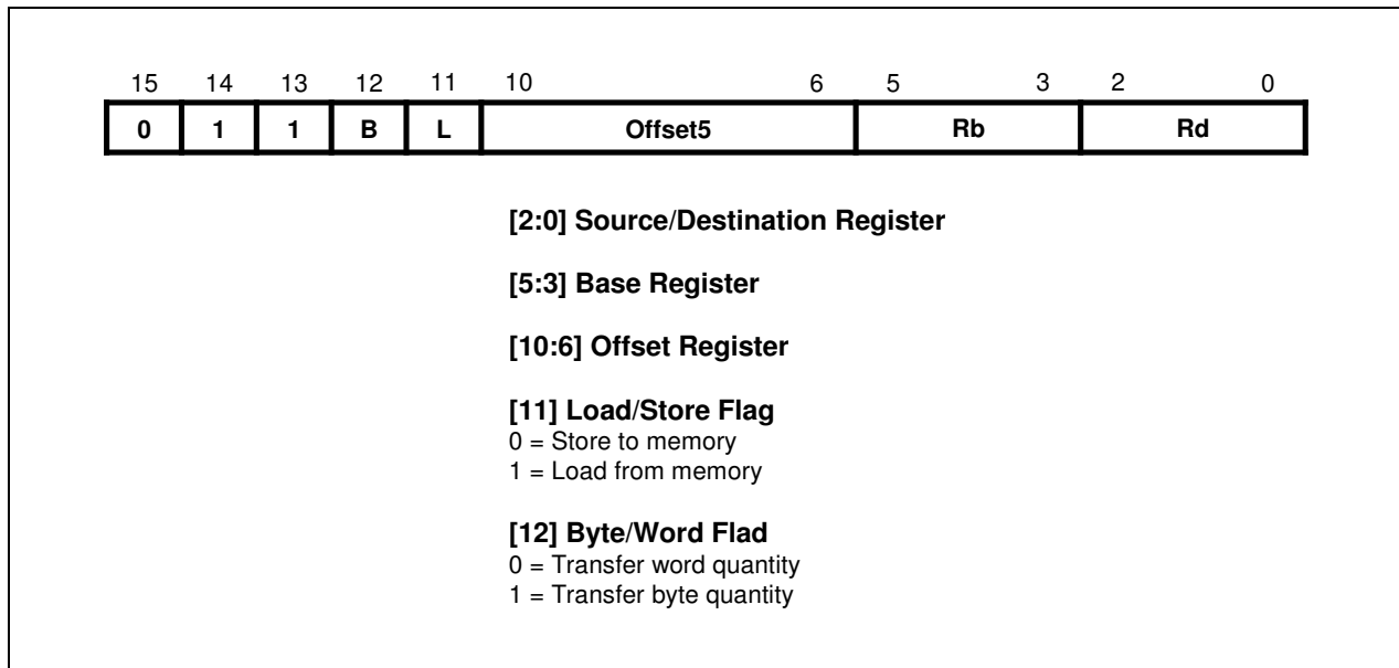
Figure 4-10. Format 9
