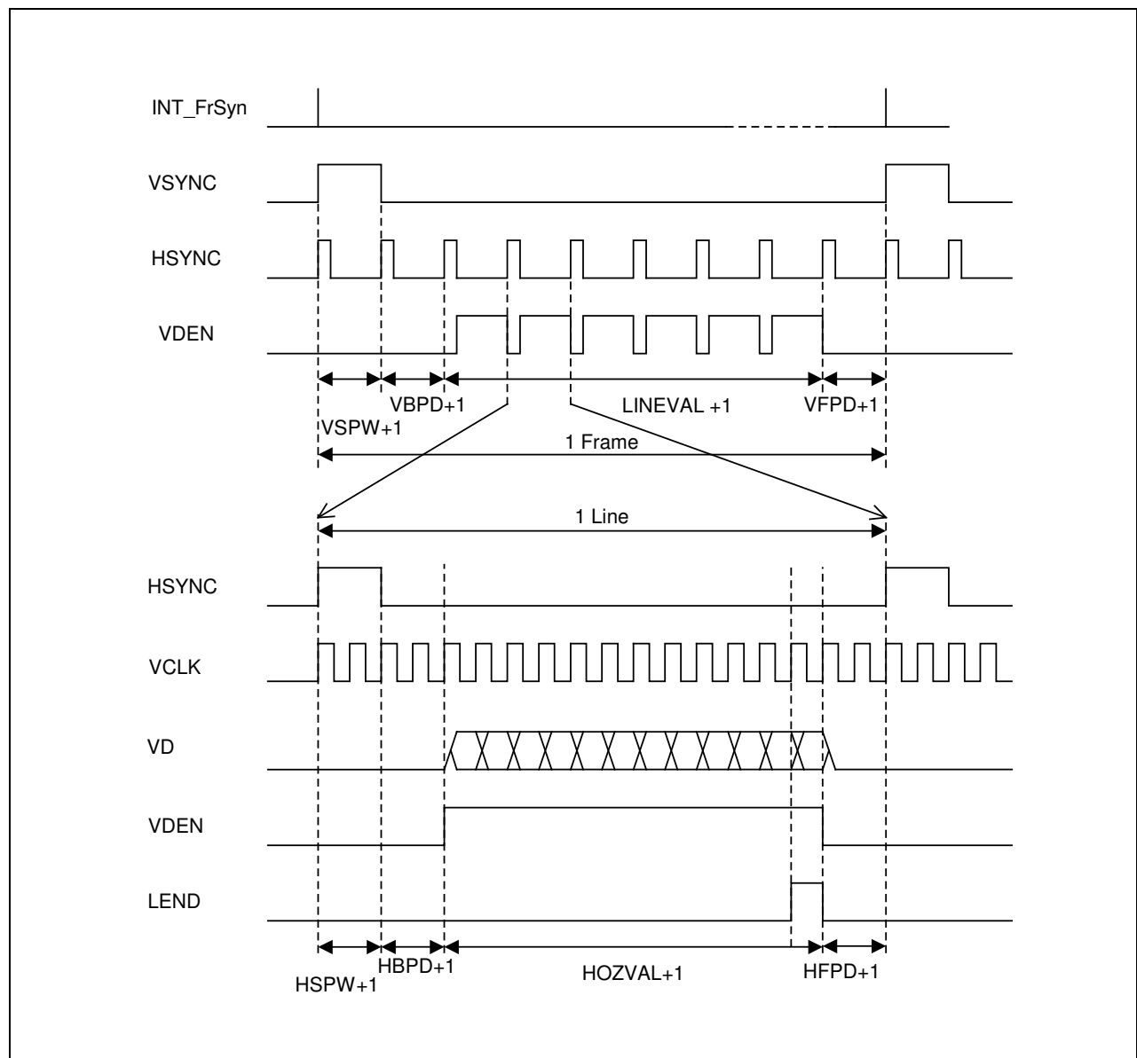
Figure 15-6. TFT LCD Timing Example
