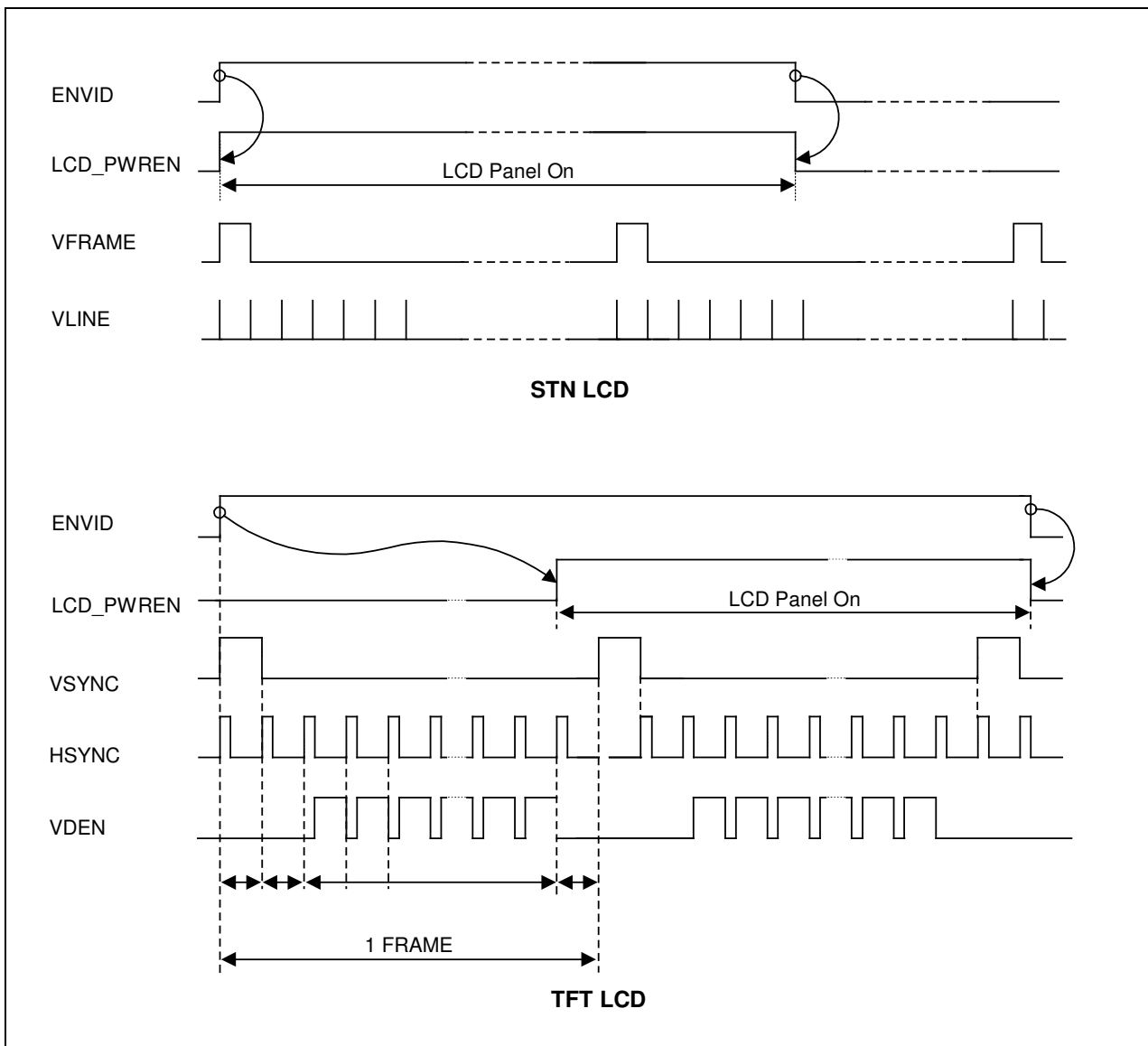
Figure 15-8. Example of PWREN Function (PWREN=1, INVPWREN=0)
