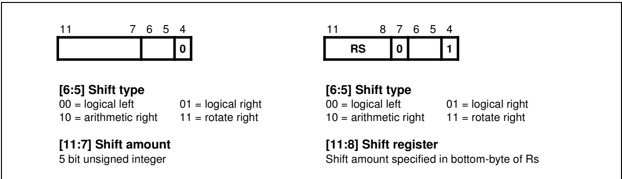
Figure 3-5. ARM Shift Operations
