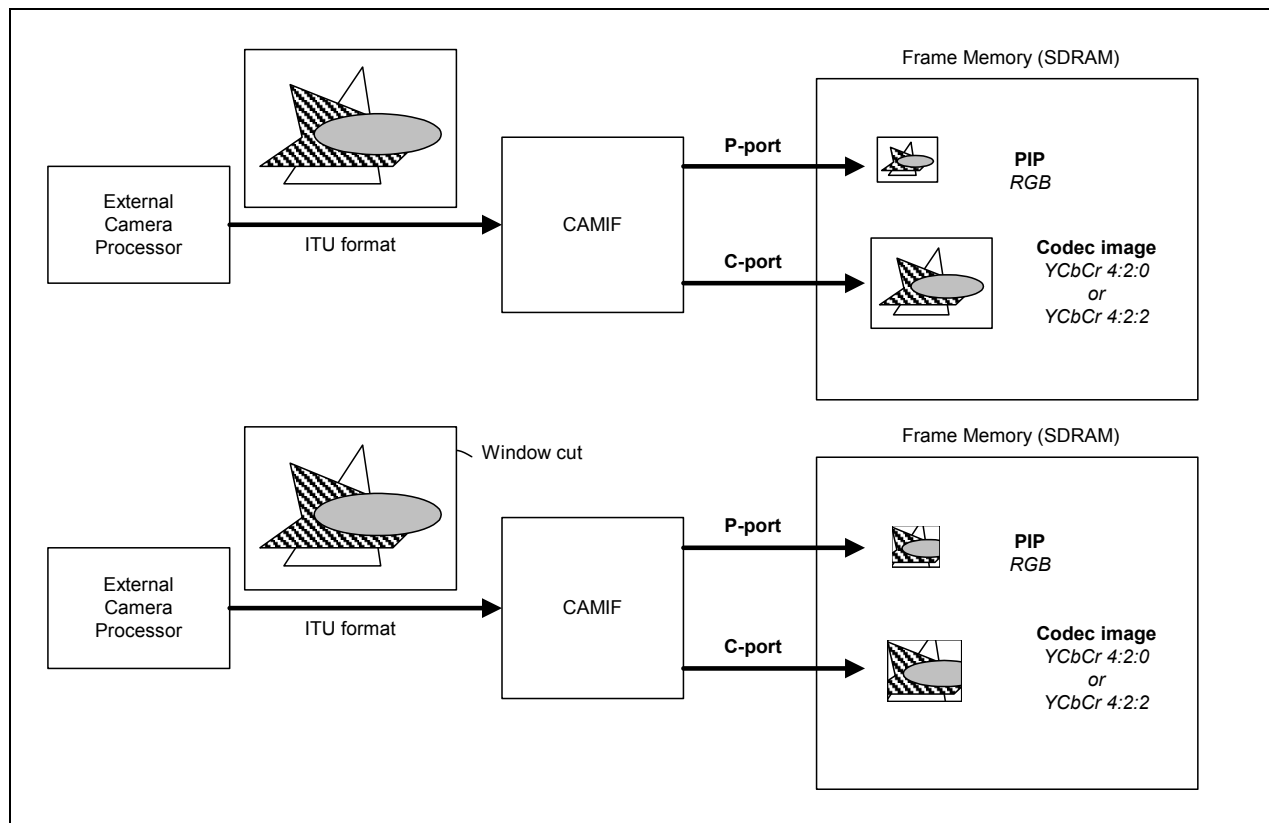
Figure 23-4. Two DMA Paths
