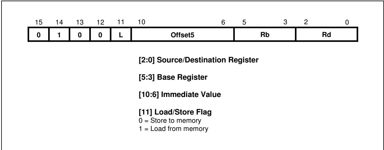
Figure 4-11. Format 10
