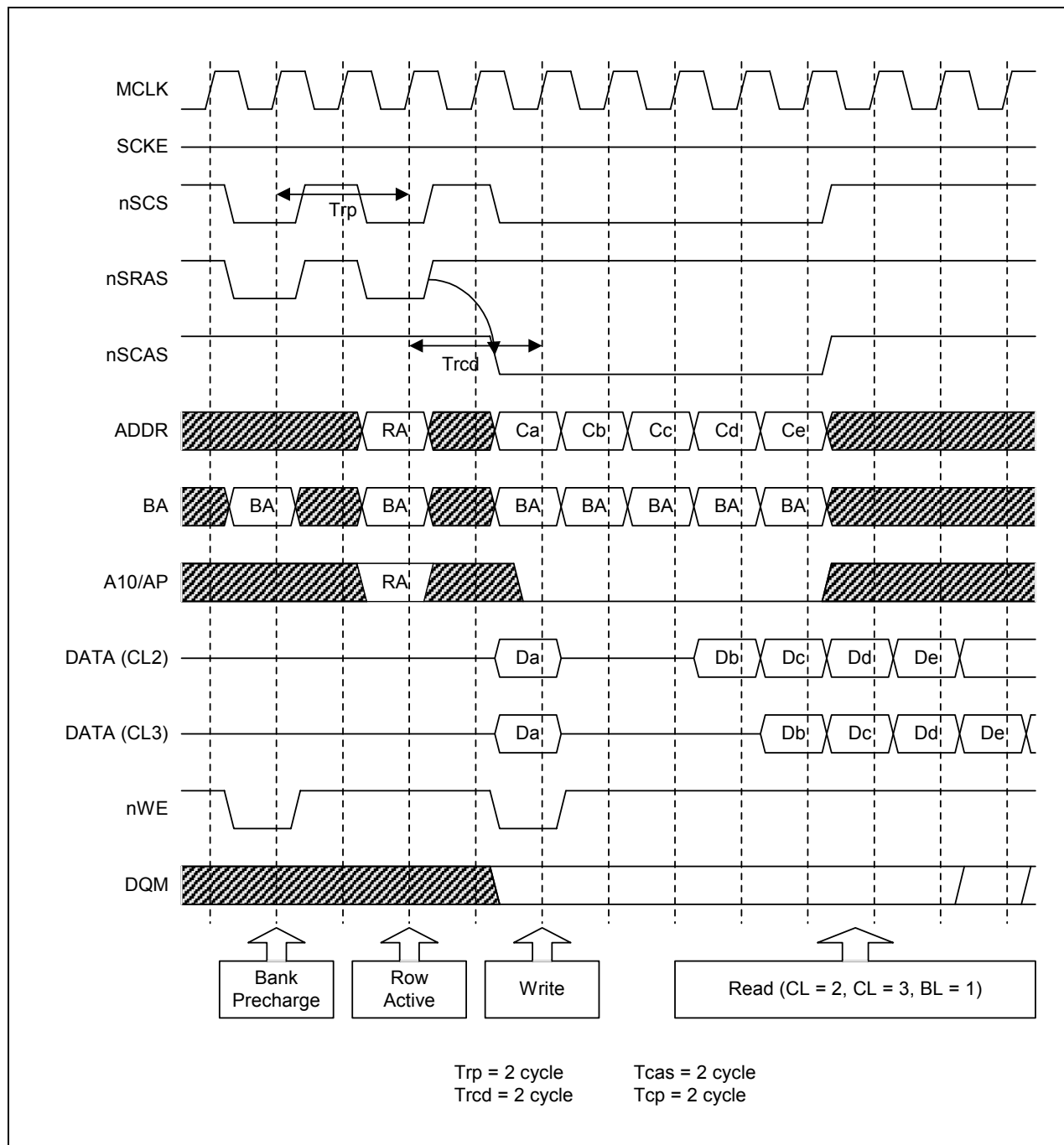
Figure 5-13. S3C2440A SDRAM Timing Diagram
