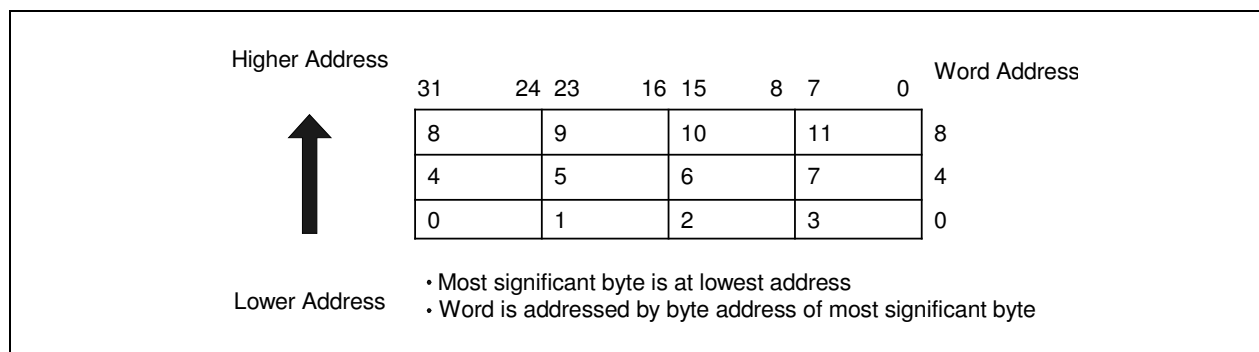
Figure 2-1. Big-Endian Addresses of Bytes within Words
