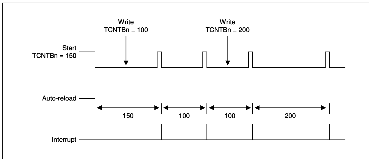
Figure 10-3. Example of Double Buffering Function
