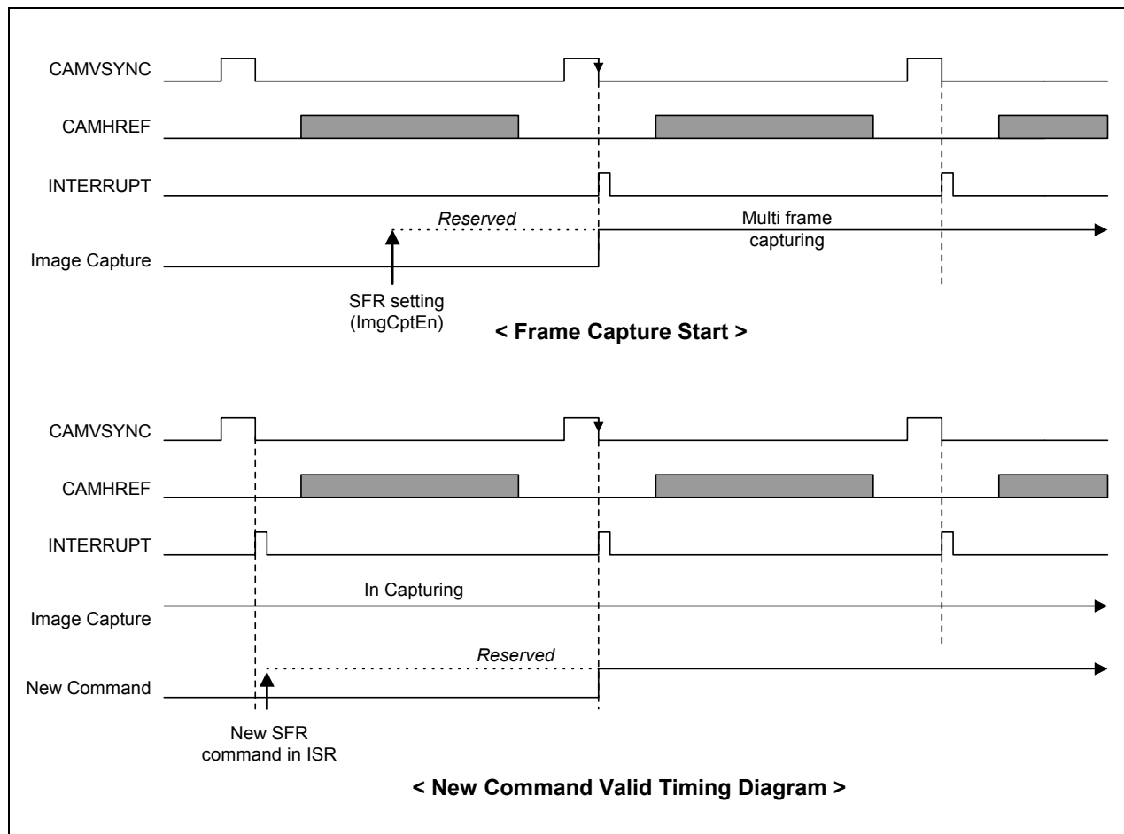
Figure 23-8. Timing Diagram for Register Setting
