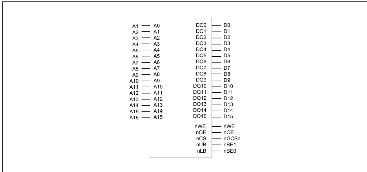
Figure 5-8. Memory Interface with 16-bit SRAM
