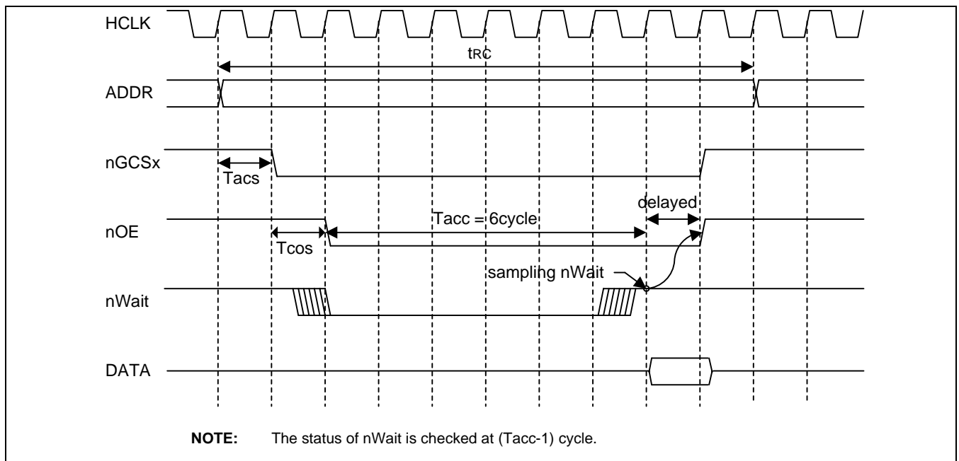
Figure 27-16. External nWAIT READ Timing Diagram (Tacs=1, Tcos=1, Tacc=4(6-cycle), Toch=0, Tcah=0, PMC=0, ST=0)
