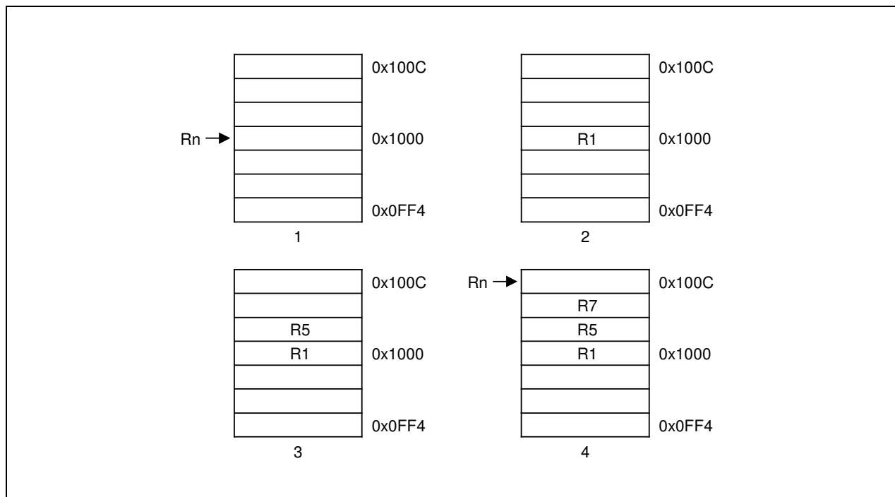
Figure 3-19. Post-Increment Addressing
