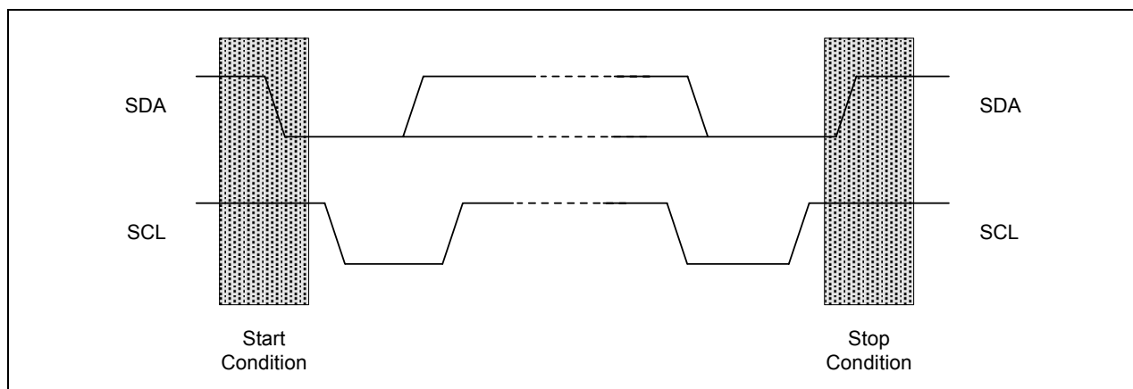
Figure 20-2. Start and Stop Condition
