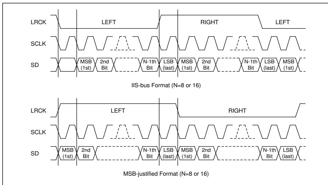
Figure 21-2. IIS-Bus and MSB (Left)-justified Data Interface Formats
