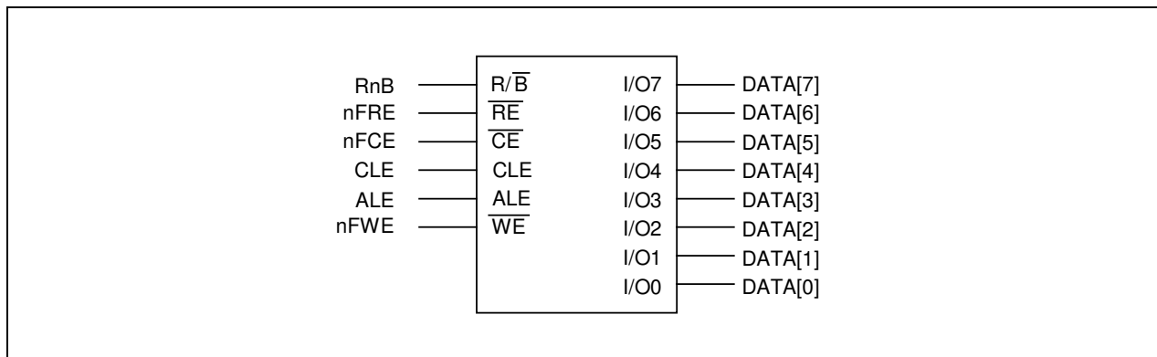
Figure 6-6. A 8-bit NAND Flash Memory Interface
