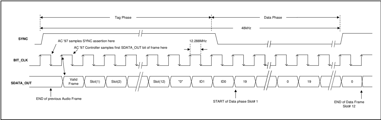
Figure 24-5. AC-link Output Frame
