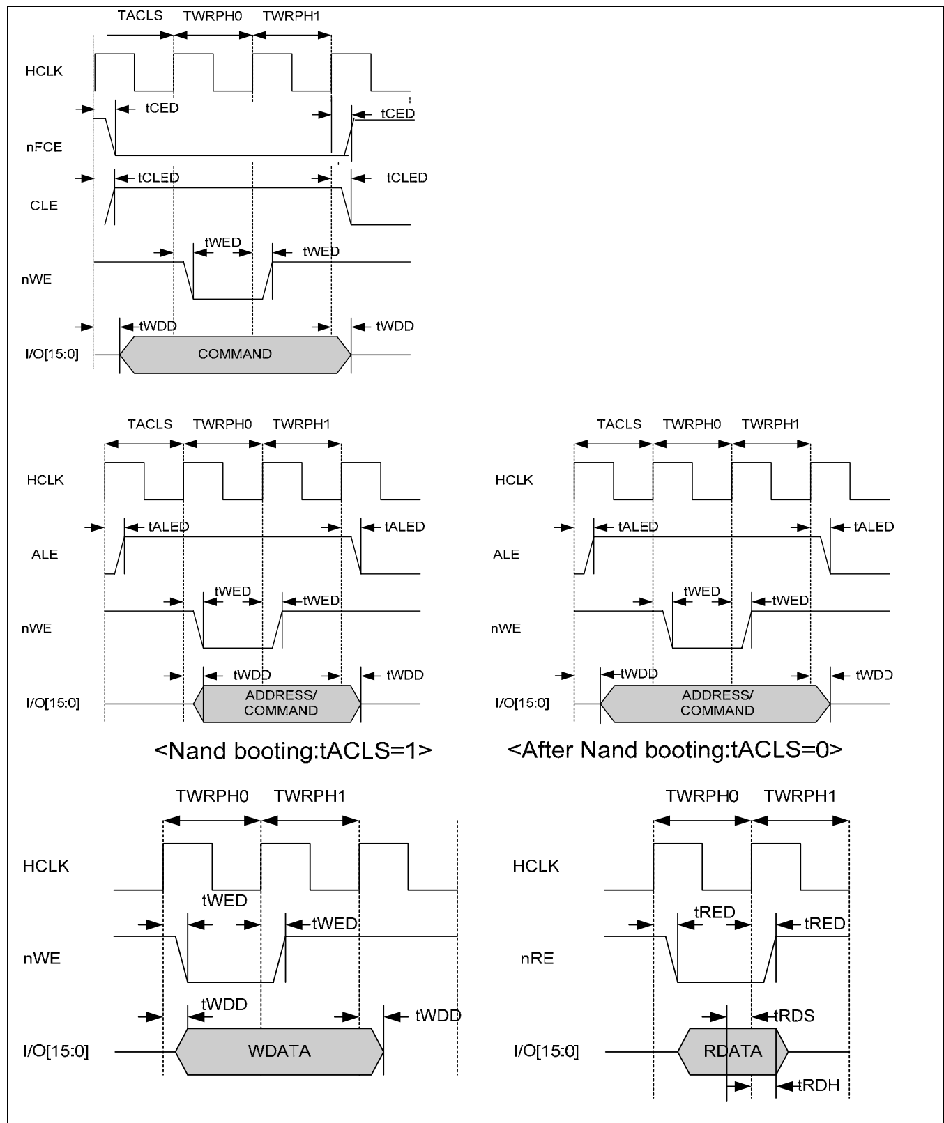
Figure 27-36 NAND Flash Address/Command Timing Diagram
