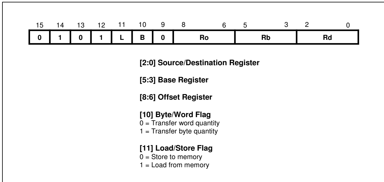
Figure 4-8. Format 7
