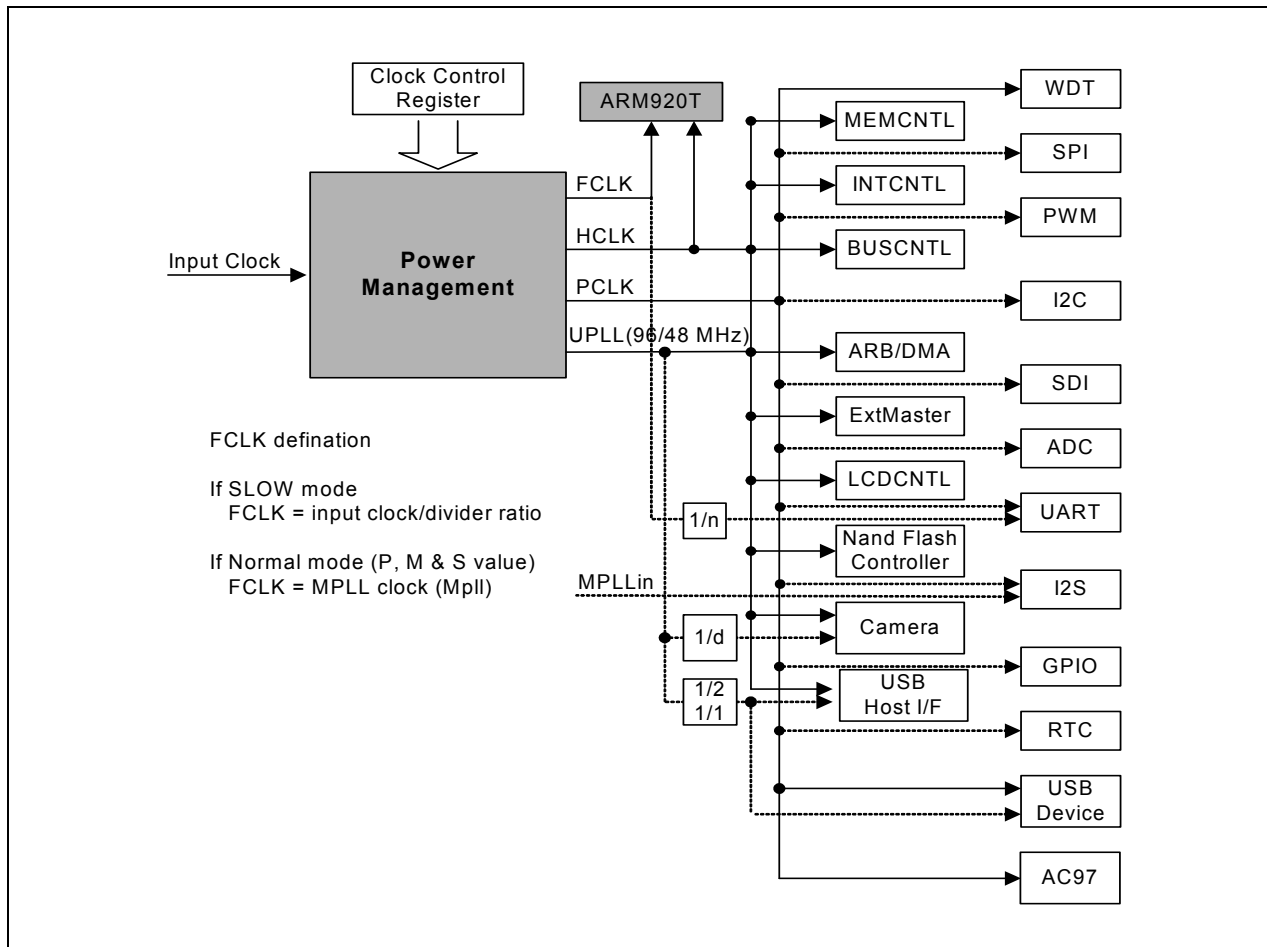
Figure 7-7. The Clock Distribution Block Diagram
