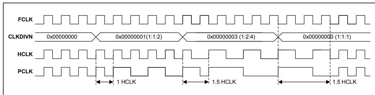
Figure 7-6. Example of Internal Clock Change
