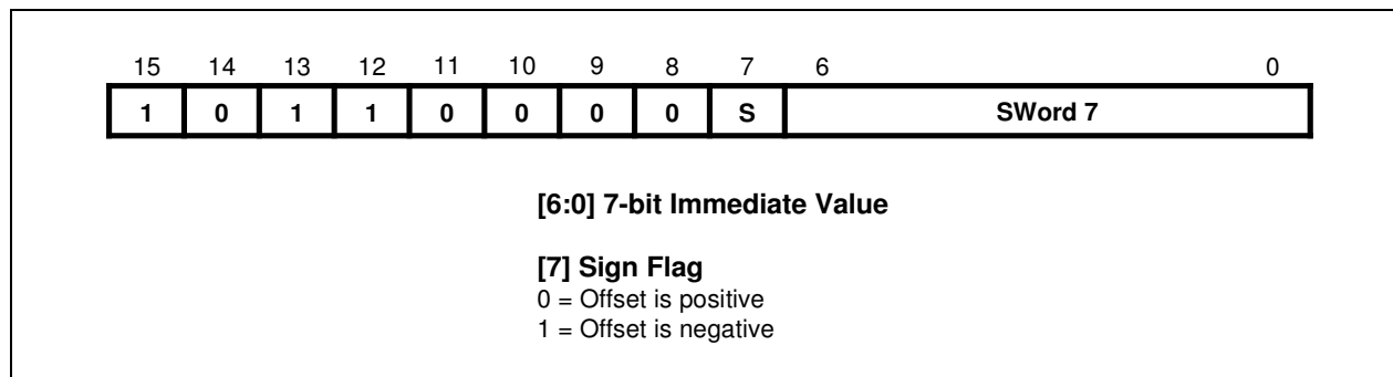
Figure 4-14. Format 13
