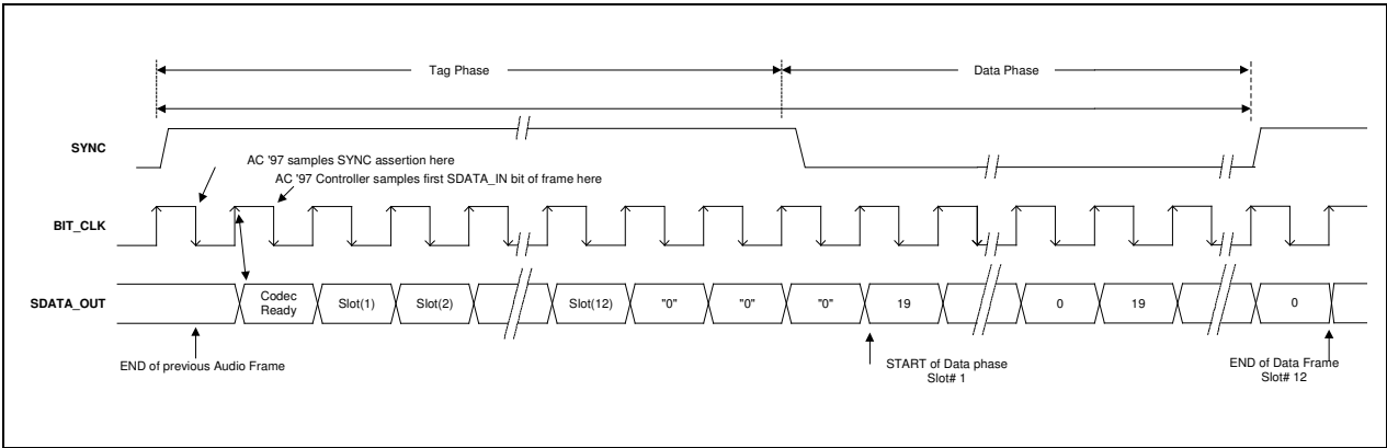
Figure 24-6. AC-link Input Frame
