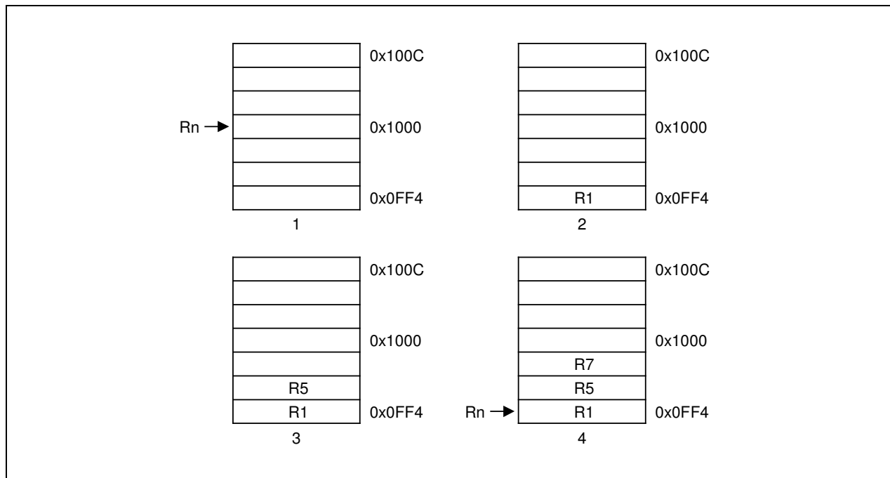
Figure 3-22. Pre-Decrement Addressing
