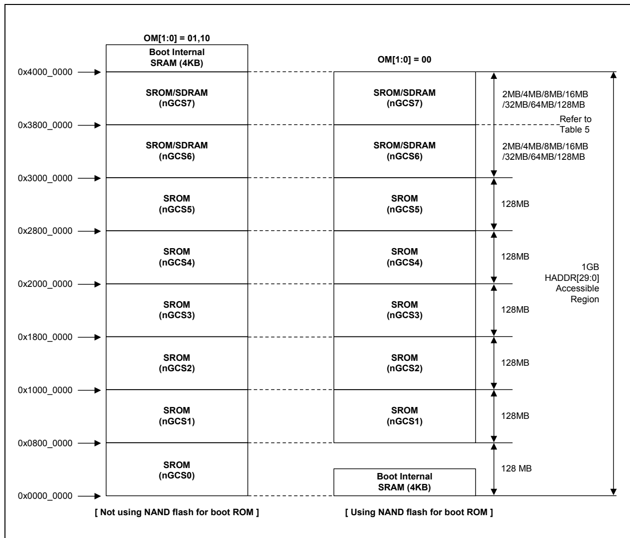
Figure 5-1. S3C2440A Memory Map after Reset
