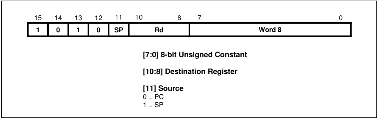
Figure 4-13. Format 12
