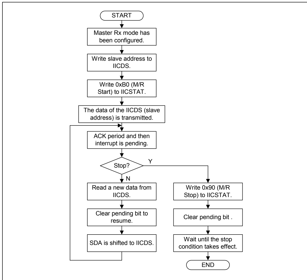
Figure 20-7. Operations for Master/Receiver Mode
