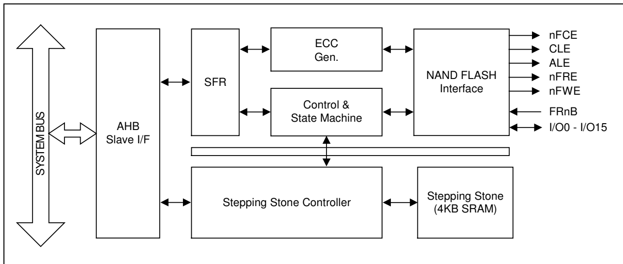
Figure 6-1. NAND Flash Controller Block Diagram
