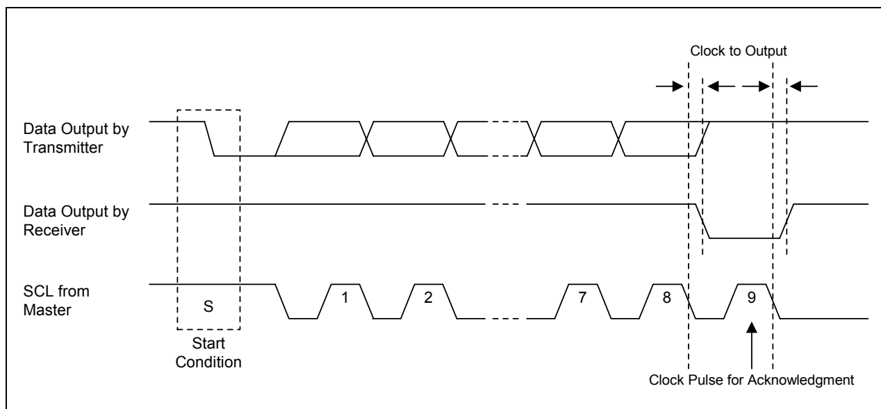
Figure 20-5. Acknowledge on the IIC-Bus
