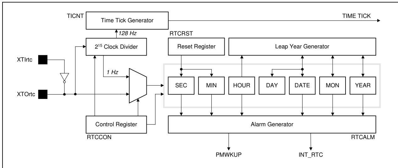
Figure 17-1. Real Time Clock Block Diagram
